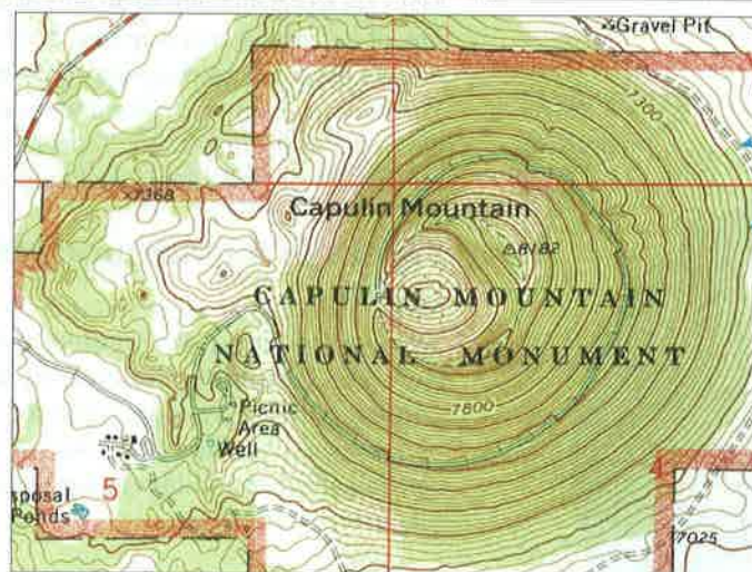
C. TOPOGRAPHIC MAP: a flat representation of Earth's surface showing horizontal positions of features plus elevations of the landscape.
