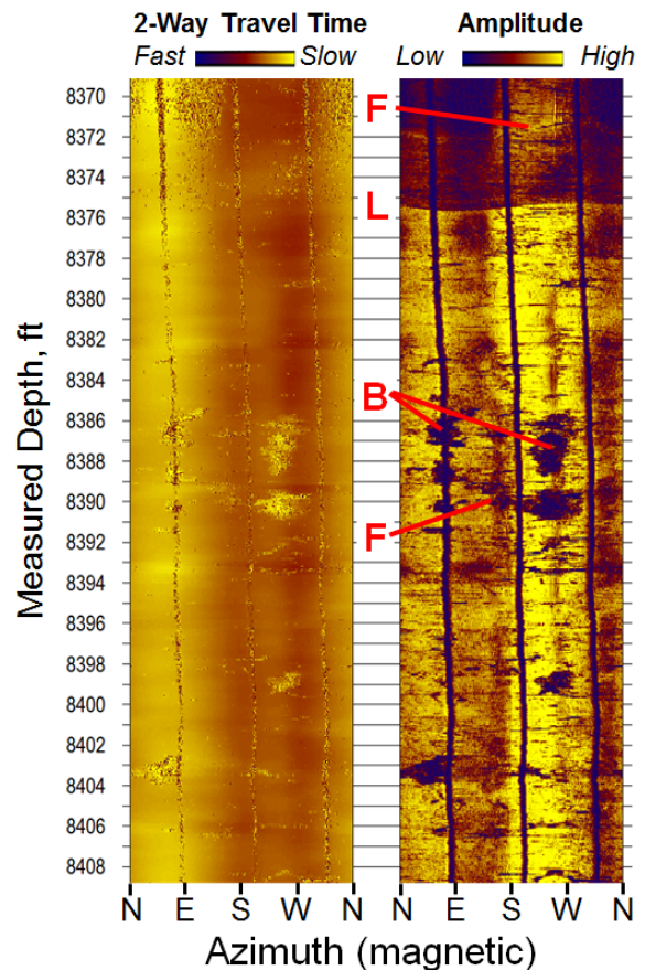
Figure 2: BHTV image from October 2010 logging of well NWG 55-29, processed to display two-way travel time (left) and amplitude (right) of the reflected ultrasonic pulse. Characteristic features are labeled as L=lithological contact, F=natural fracture, and B=borehole breakout. The three dark, vertical bands are not natural features in the borehole, but rather are shadows produced by structural rods attached to the BHTV.
