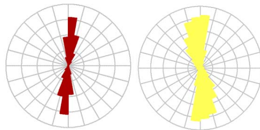
Figure 5: Rose diagram of LiDAR scarps (left) and fissures (right) mapped in Figure 4.
