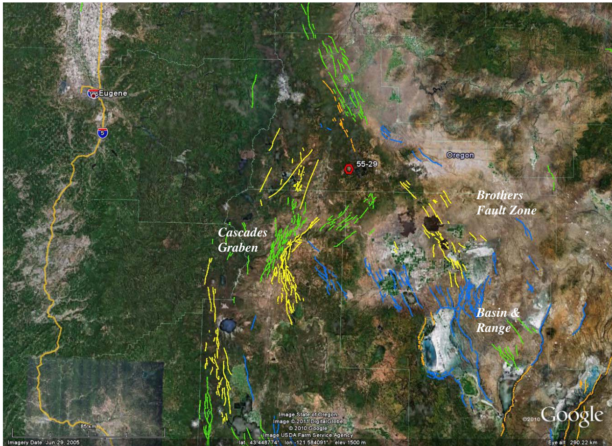
Figure 1: Regional Map showing location of the Newberry EGS demonstration site (well NWG 55-29) at the intersection of three structural trends in central Oregon. Colored lines are faults from the USGS Quaternary fold and fault database. The fault ages are coded by color, from oldest to youngest: blue, green, yellow, orange.
