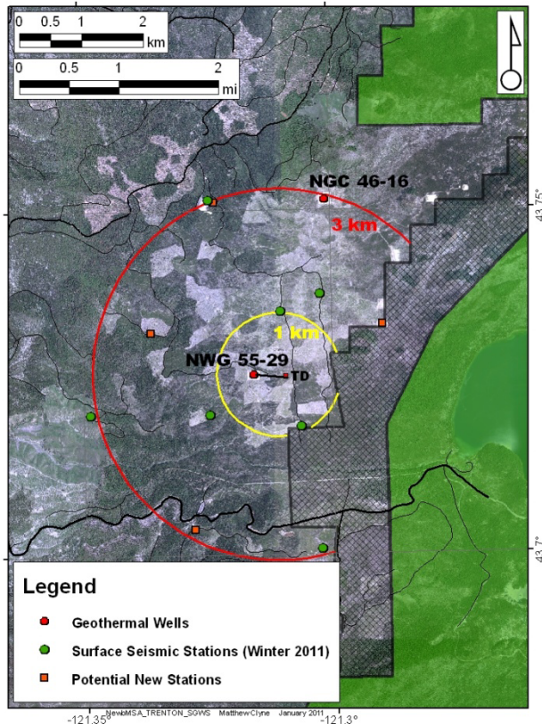
Figure 3: EGS Project's Microseismic Array (MSA), centered on the EGS injection well NWG 55-29. TD marks the bottom of the well which is deviated to the east.
