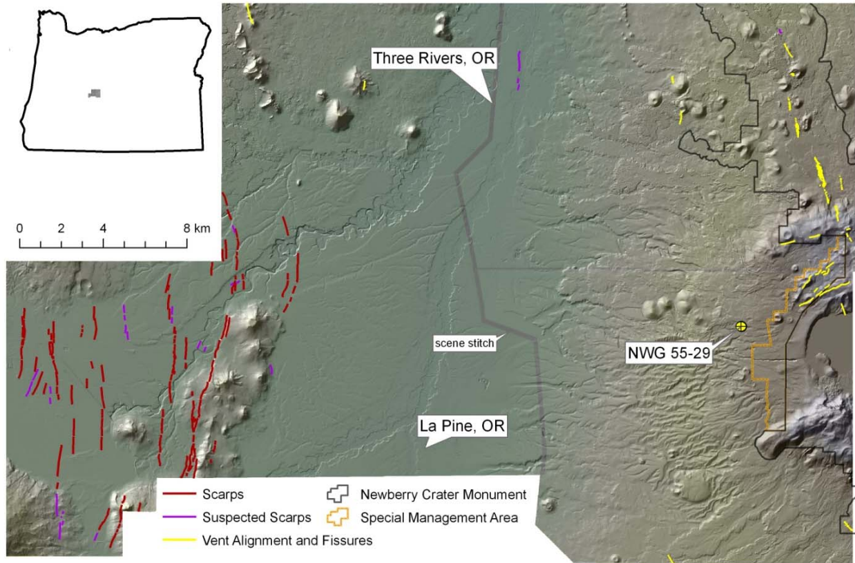
Figure 4: Oregon LiDAR Consortium image from the west flank of Newberry Caldera. Fault interpretations shown are by ARE.
