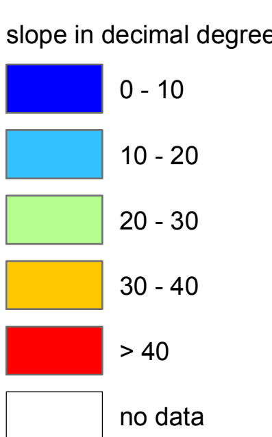
Slope Map
