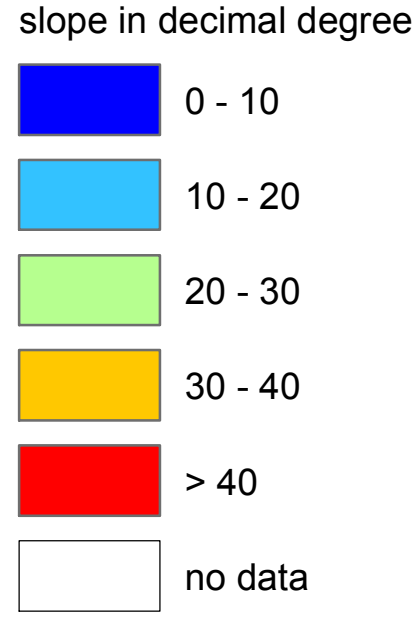
Slope Map
