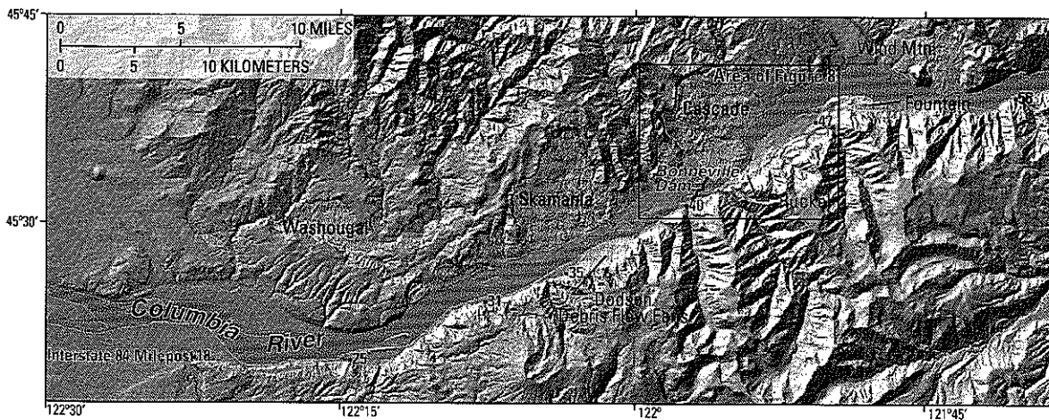
Figure 3. Landslides and landslide complexes of the western Columbia River Gorge, after Palmer (1977).
