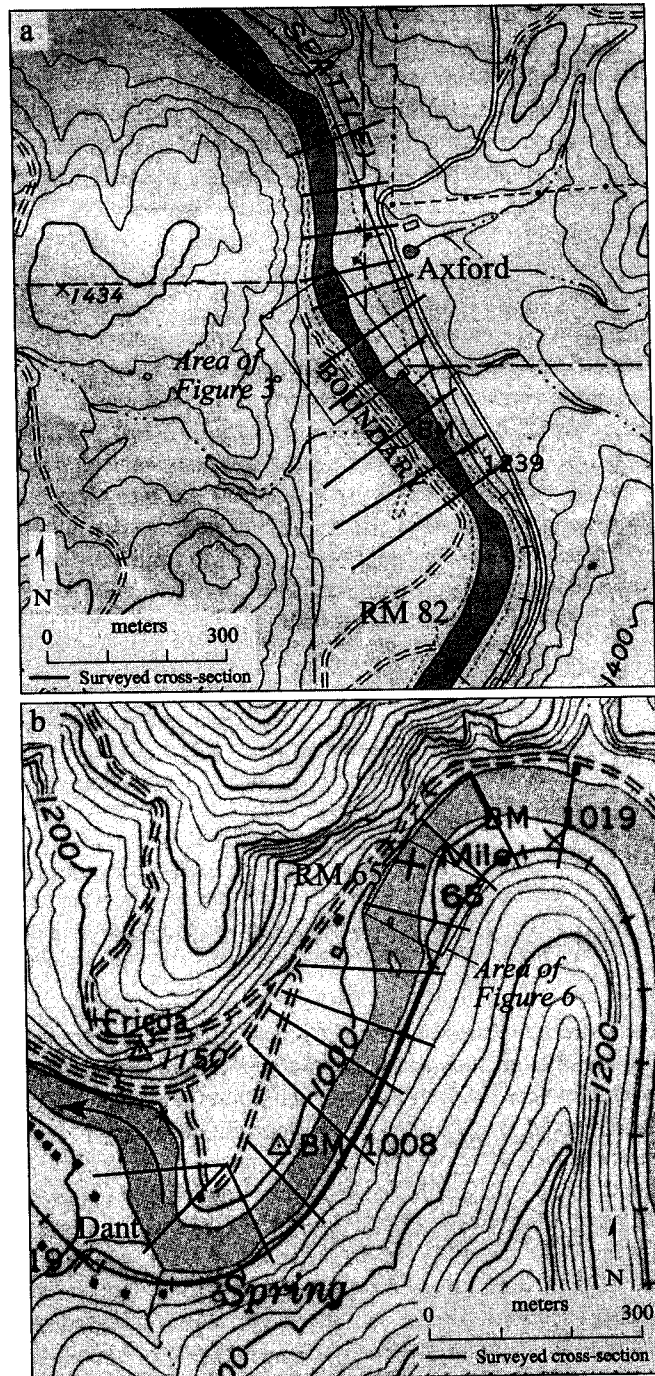
Figure 14. Maps of (a) Axford and (b) Dant study reaches, showing surveyed cross-sections used for hydraulic modeling. Topographic base from the Kaskela and Dant, Oregon, USGS 7.5-minute topographic quadrangles. Contour interval is 12 meters (40 feet).
