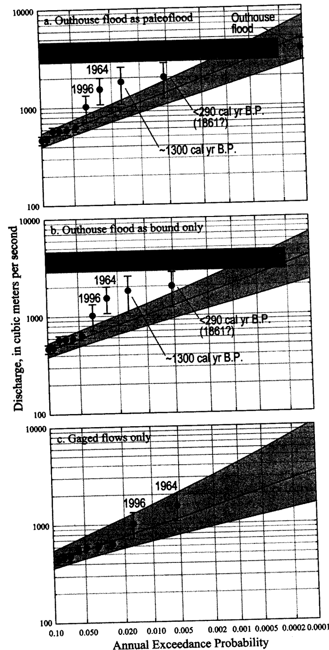
Figure 17. Plotting positions and flood-frequency analysis for gaged floods and paleofloods on the Deschutes River, calculated using the Bureau of Reclamation FLDFRQ3 program [O'Connell, 1998; O'Connell et al., 2002]. Plotting positions calculated using the Hazen method. Flood-frequency analyses were conducted for log 10 Pearson Type III distributions. For all cases, gaged discharges greater than 700 m 3 /s (adjusted for the Axford study site) were assumed to have fractional 2σ standard errors of 0.3, except for the value for the 1964 flood, which was also adjusted for effects of regulation and assigned a fractional 2σ standard error of 0.5. Gaged flows less than 700 m 3 /s were assigned fractional 2σ standard errors of 0.1. The discharges, ages, and likely ranges of paleoflood data were prescribed as shown in Table 2. In all cases, the "best estimate" of Table 2 was assumed to be 10 times more likely than the minimum and maximum estimates, thus providing an estimate of the shape of the probability distribution about the true discharge. Plots (a) and (b) summarize results of analyses that include the 94 years of gaged annual floods, the <290 and ~1300 cal yr BP paleofloods, and the non-exceedance bound provided by the ~4600-yr old Outhouse flood deposits. Plot (a) also includes the Outhouse flood as a paleoflood, whereas (b) only includes it as a non-exceedance bound, accounting for the possibility that the Outhouse flood was generated by a non-meteorological event. Plot (c) summarizes results from a similar analysis including only the 94 years of gaged flows.
