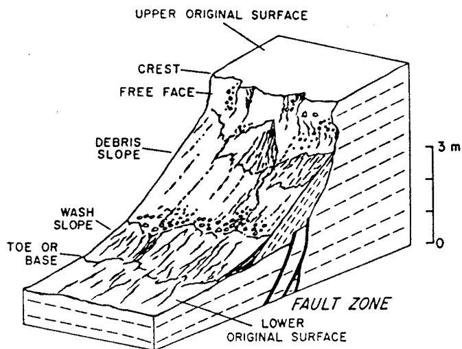
Block diagram of a fault scarp showing terminology used in this study.
