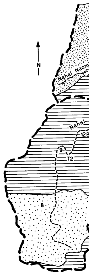
FIG. 2. Geology and location of study area, Nahal Yael watershed, Shimron (Schick and Sharon, 1974).
