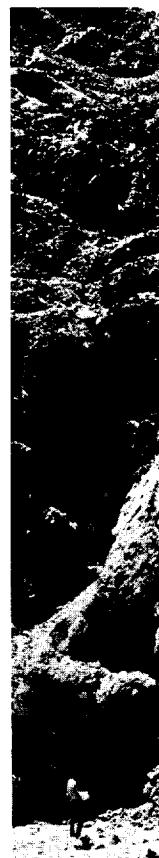
FIG. 9. Colluvium derived from m source area for the colluvium and s
