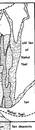
Map of colluvium (the areas of smooth
