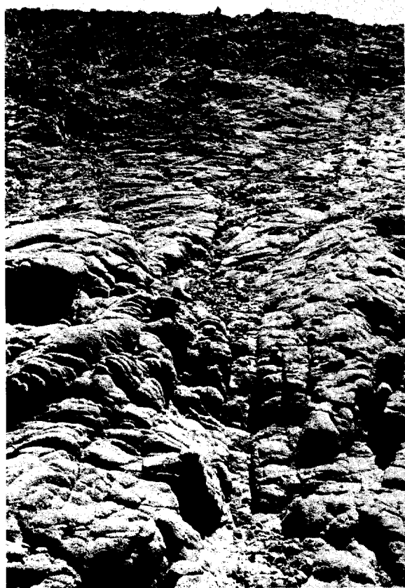
FIG. 3. North-facing hillslope of Elat granite with contrasts in smoothness of outcrops. View along transect of Figs. 6 and 7.
