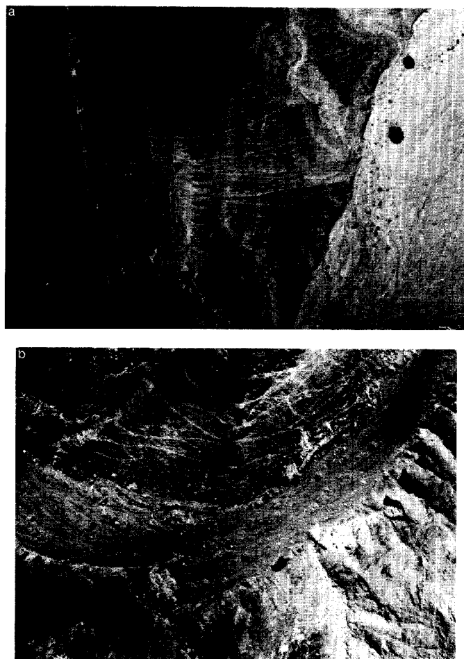
FIG. 12. Trails on surfaces that are relict from a time of wetter climate. A. The alluvial fan of Nahal Yael. B. Colluvium derived from metasedimentary rocks. C. Quartz porphyry dike in the Elat granite.
