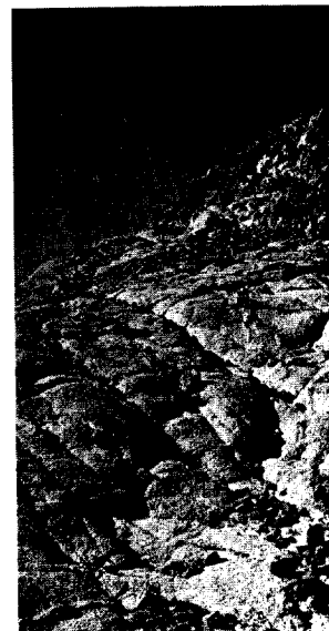
FIG. 4. North-facing hilltop of Elat granite. Hammer in center foreground for scale.
