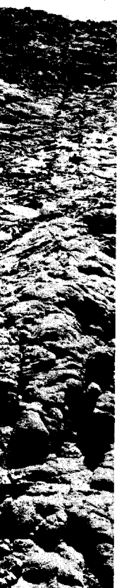
in smoothness of outcrops. View along
