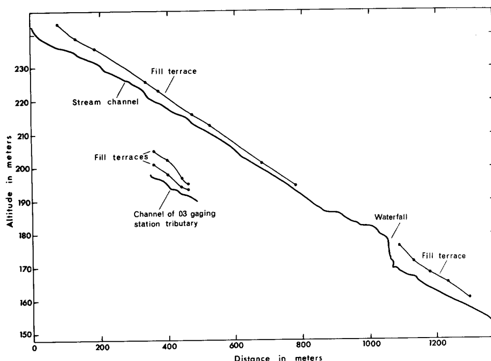
FIG. 11. Longitudinal profiles of fill terraces and stream channels of Nahal Yael.
