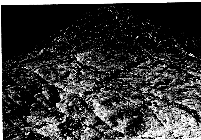
FIG. 4. North-facing hilltop of Elat granite with contrasts in smoothness of outcrops. Hat in left center foreground for scale.
