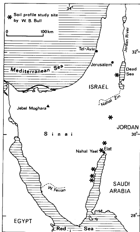
FIG. 1. Map of Sinai Peninsula and adjacent areas showing soil study sites.
