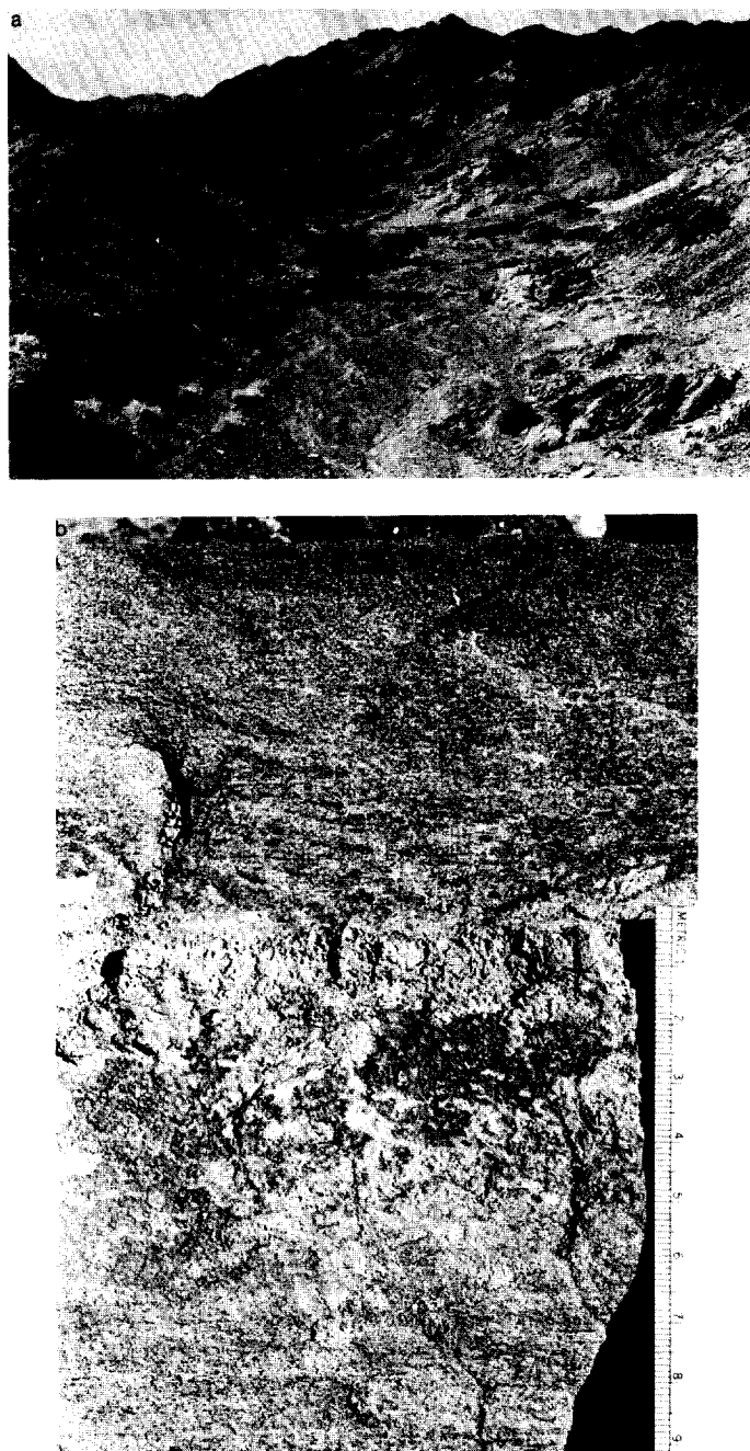
FIG. 10. A. Strath and fill terraces in Nahal Yael. B. Shallow depth of carbonate illuviation on schist boulder on early Holocene terrace. Ground level was at 0 cm. Foliation of schist is apparent above and below 6 cm band of \text{CaCO}_3 accumulation.
