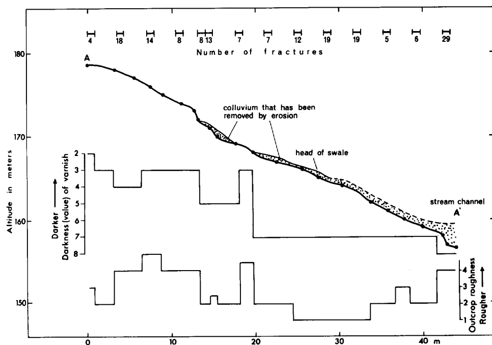
FIG. 7. Former thickness of colluvium, outcrop roughness, desert varnish, and fracture density in the Elat granite. The location of transect A-A' is shown on Fig. 6.
