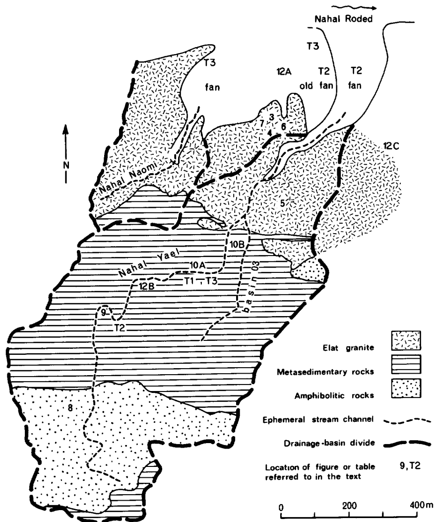
FIG. 2. Geology and location of study sites in the Nahal Yael research area. Geology chiefly from Shimron (Schick and Sharon, 1974, p. 104).
