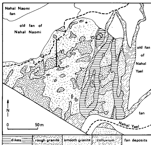
FIG. 6. Map of hillslopes of Elat granite that have been stripped of colluvium (the areas of smooth granite). Transect A-A' is shown in Fig. 7.
