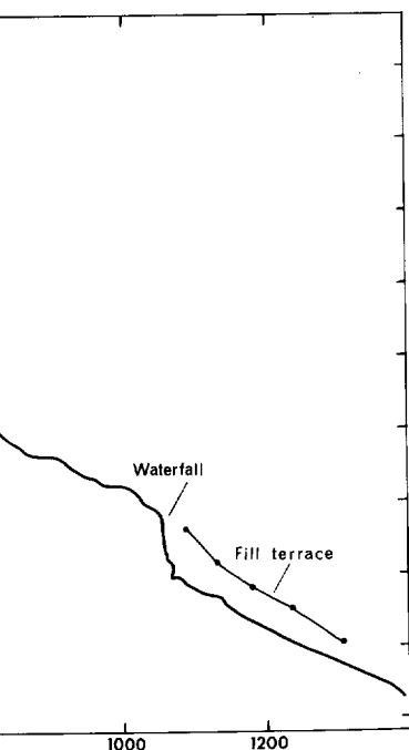
stream channels of Nahal Yael.
