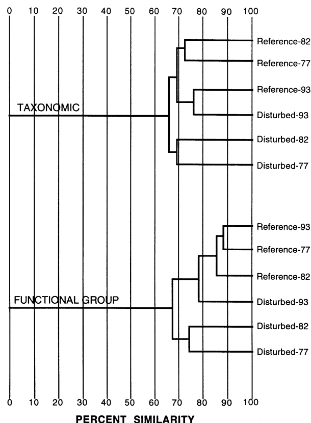
Fig. 4 Per cent similarities between reference (Hugh White Creek) and disturbed (Big Hurricane Branch) streams based on habitat-weighted abundance of Ephemeroptera, Plecoptera and Trichoptera during 1977–78, 1982–83 and 1993–94.
