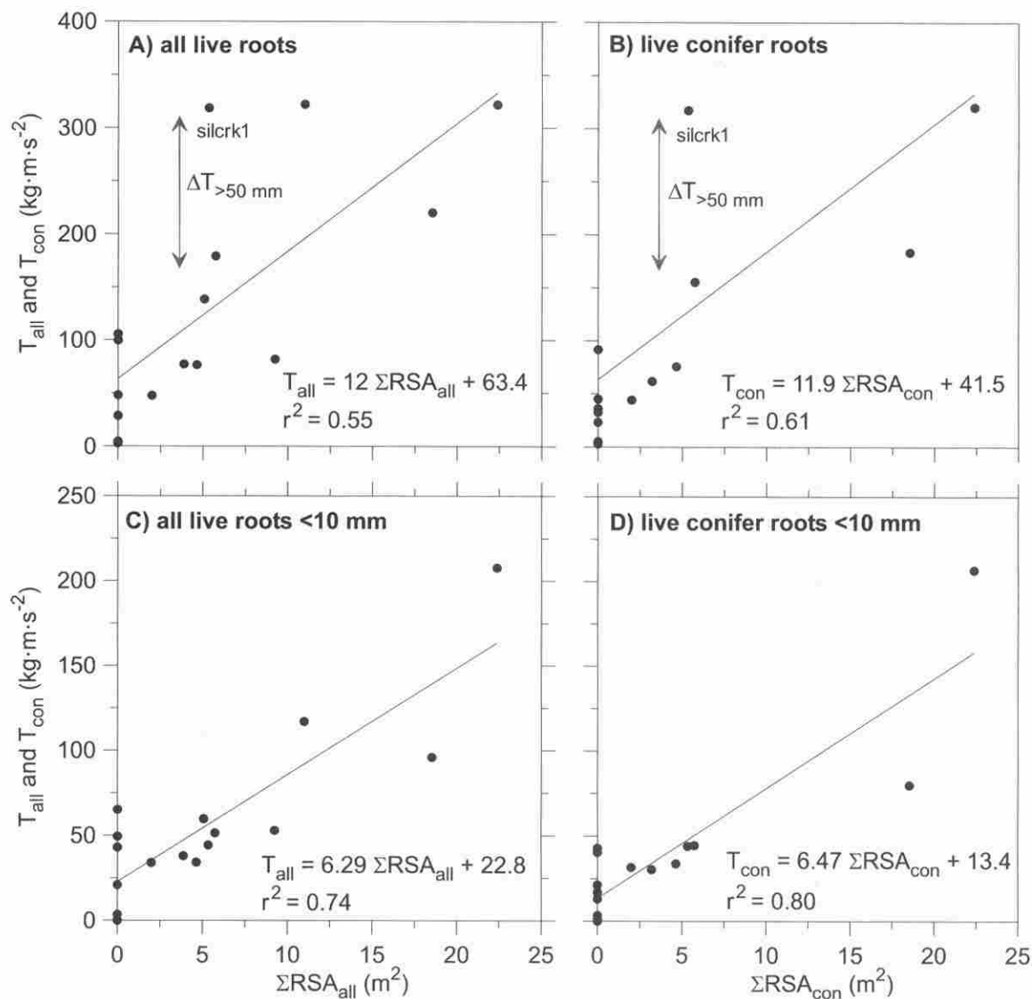
Fig. 12. Plots of total root tensile strength ( T_{all} and T_{con} ) as a function of our geometric root network factor ( \Sigma RSA ) for (A) all live trees, (B) live conifer trees, (C) all live trees and roots <10 mm in diameter, and (D) live conifer trees and roots <10 mm in diameter. The sites are described in Table 1 (see Schmidt et al. (2001) for details on tensile strength calculation). A positive correlation is observed for all four datasets. The thin black lines are linear regression fits and the associated equations are shown on the graph. At some sites (particularly silcrk1), a significant fraction of the root strength results from a limited number of large-diameter roots. The thick gray vertical arrows in (A) and (B) labeled with \Delta T_{>50mm} denote the amount of root strength attributed to two conifer roots with diameter >50 mm at the silcrk1 site.
