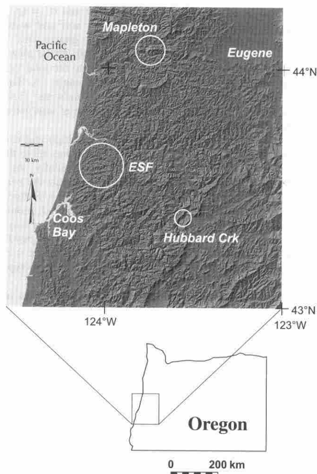
Fig. 1. Location figure of OCR showing the location of our three study areas: Mapleton, ESF (which includes Silver Creek stand), and Hubbard Creek. We analyzed: 21 landslides in Mapleton, 11 landslides and 2 soil pits in ESF, and 2 soil pits in Hubbard Creek. For further data on the Mapleton and ESF sites, see Robison et al. (1999).
