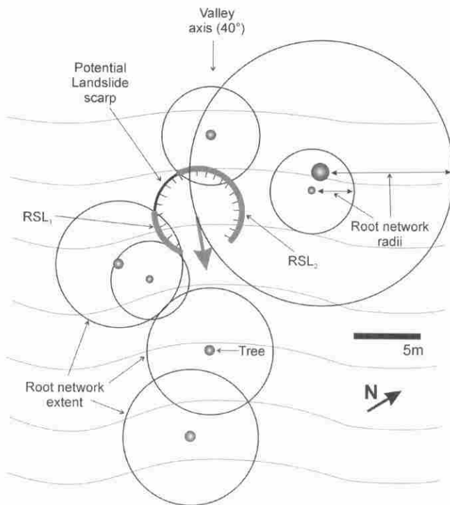
Fig. 13. Planview map of an unchanneled valley in the Mapleton study area that did not fail during the 1996 storms. The distribution of trees and root networks (calculated with eq. [3]) most relevant to slope stability are plotted. Gray lines are topographic contours that depict a topographic hollow in the center that drains downward. Douglas-fir tree trunks and their associated root networks are indicated by fill-shaded gray circles and black circles, respectively. Through an iterative search, the location of a landslide scarp (with an effective radius of 3 m) that minimizes \Sigma RSL is shown by the hachured circular arc, wherein the total arc length of the scarp intersected by root networks ( \Sigma RSL = RSL_1 + RSL_2 ) is 11.6 m. See text for description of how this value is converted to root cohesion and incorporated into a slope stability analysis.
