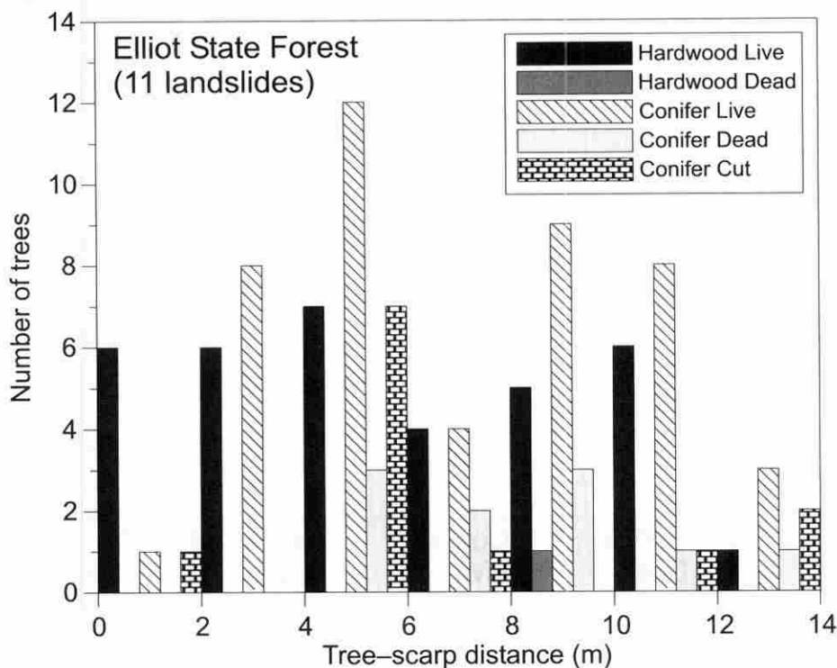
Fig. 5. Histogram describing the tree-to-scarp distance, d_s , for all trees within 14 m of 11 landslides in the ESF study area. See text for species included in hardwood and conifer categories. Note the approximately equal numbers of live hardwood and coniferous trees adjacent to landslide scarps.
