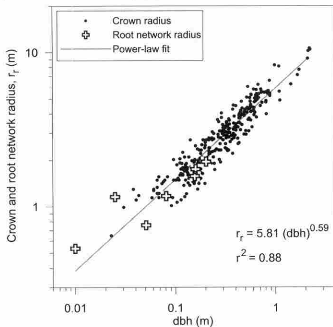
Fig. 10. Log-log plot illustrating the relationship between dbh (m) and crown and root network radius (m) of Douglas-fir trees. Crown and root network radii are well-correlated (McMinn 1963; Smith 1964), such that crown radius can be used to approximate root network radius. Crown radius points were obtained from Maguire (personal communication, 2000) and from our field measurements. Root network radius values were given by McMinn (1963). Root network and crown radius varies as a power function of dbh (eq. [3]).
