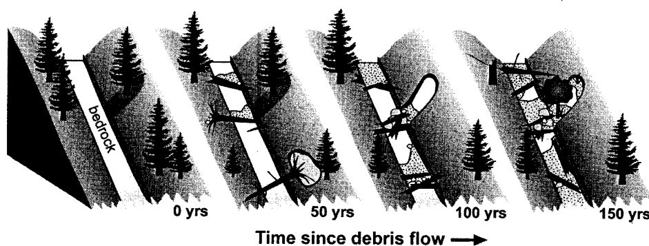
Figure 5. Conceptual illustration of the changes in channel morphology based on the time since the previous debris flow
