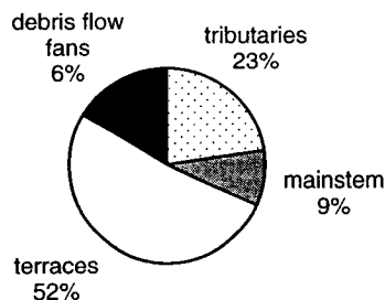
Figure 9. The proportion of sediment stored in the channel network and valley floor landforms of Skate Creek
