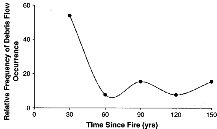
Figure 10. Debris flow activity in the immediate post-fire and inter-fire time periods in Skate and Bear Creeks. Data are grouped into 30 year age classes and the trend line was added to illustrate the overall pattern
