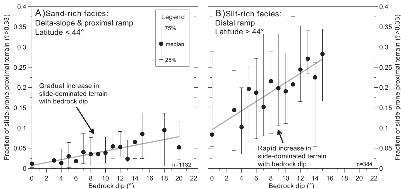
Figure 11. Variation in the fraction of slide-prone terrain with bedrock dip angle for (A) sand-rich facies south of 44^\circ latitude, and (B) silt-rich facies north of 44^\circ latitude. For each strike and dip observation ( n = 1516 ), we calculated the fraction of surrounding terrain (within 2.5 km) with \beta > 0.33 . Each data point represents the median value for 1^\circ bins of bedrock dip angle. Upper and lower error bars represent the 75th and 25th percentile values, respectively. The extent of failure-prone terrain increases linearly with dip in both regions, although the silt-rich areas exhibit a higher proportion of landslide-prone terrain for a given bedrock dip angle. Summary statistics for linear regressions fit to the median values are: y = 0.0035x + 0.0077 , r^2 = 0.65 for the sand-rich region and y = 0.0116x + 0.096 , r^2 = 0.81 for the silt-rich region. We did not calculate median values for bins with fewer than 10 data points.
