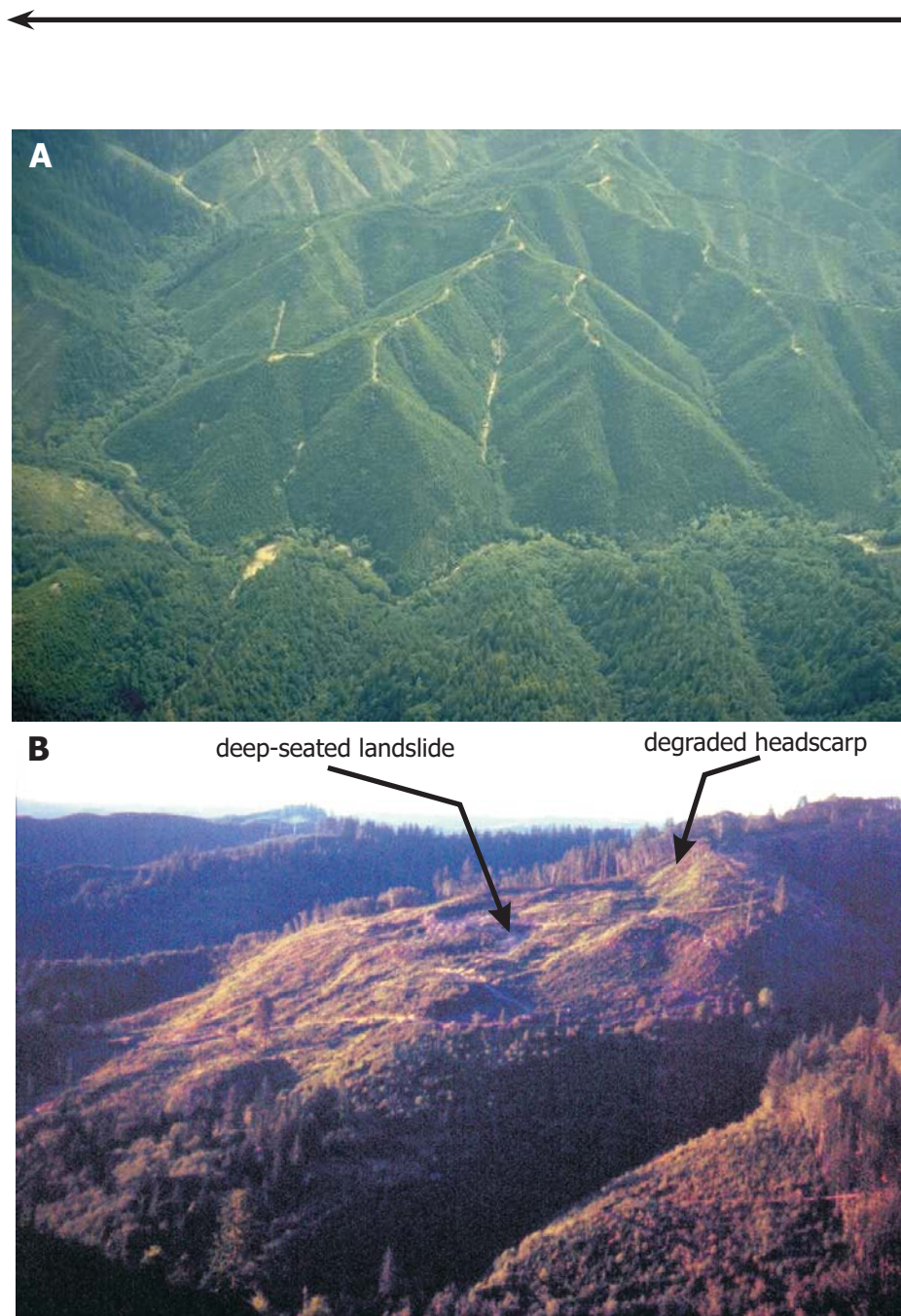
Figure 3. Oblique photos of (A) steep and dissected terrain often cited as characteristic of the Oregon Coast Range (OCR), and (B) an ancient deep-seated landslide in the OCR (latitude: 43.47°N, longitude: 124.12°W) that exhibits a low-gradient, benchlike morphology.
