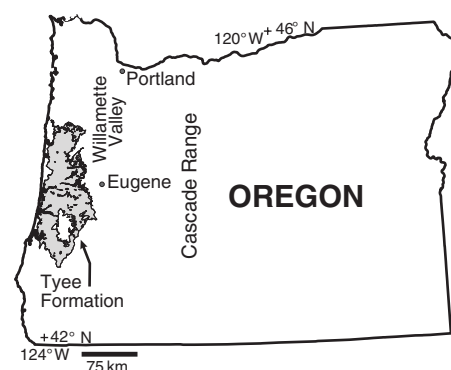
Figure 1. Location map of the Tyee Formation (Eocene sedimentary rocks) in the central Oregon Coast Range.
