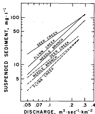
Fig. 7. Monthly suspended sediment concentrations and monthly stream discharge (1959–1965 WY). Solid lines show fall and winter months before and including the seasonal peak discharge. Dashed lines show winter and spring months after the seasonal peak discharge.
