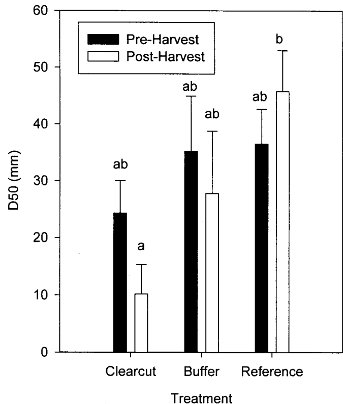
Figure 8. Results of Two-Way (time x treatment) ANOVA of the Median Particle Diameter in the Channel Bottom. Bars show mean of each group and error bars show the standard error of the mean. Groups which do not share a letter are significantly different according to Tukey multiple comparison. The median particle diameter was determined from sieving three grab samples collected at the same randomly-selected locations before and after harvest.
