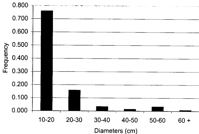
Figure 9. Histogram of Diameters of Large Woody Debris Left in the Clearcut Streams After Yarding. Distribution determined by stretching a tape longitudinally over the channel and measuring the diameter of each piece of wood greater than 10 cm diameter touched by the tape.
