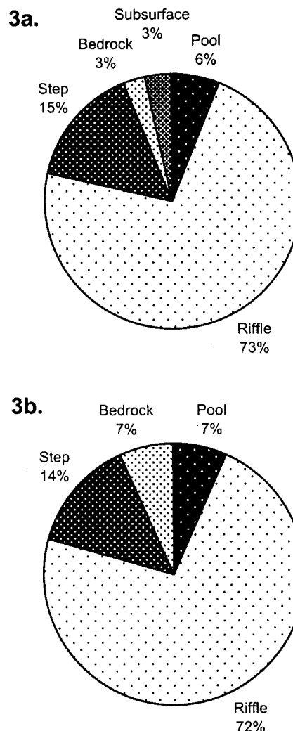
Figure 3. Comparison of (a) Pre-Harvest and (b) Post-Harvest Habitat Distributions in the Four Reference Streams Based on Longitudinal Channel Distance.
