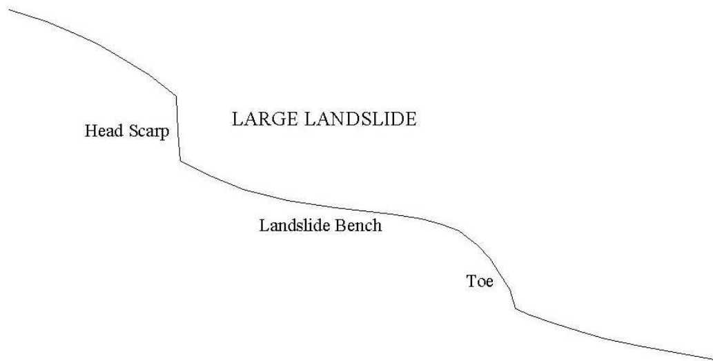
Figure 1. Shape of deep-seated landslide; scale on order of 50 to 1000 feet.
