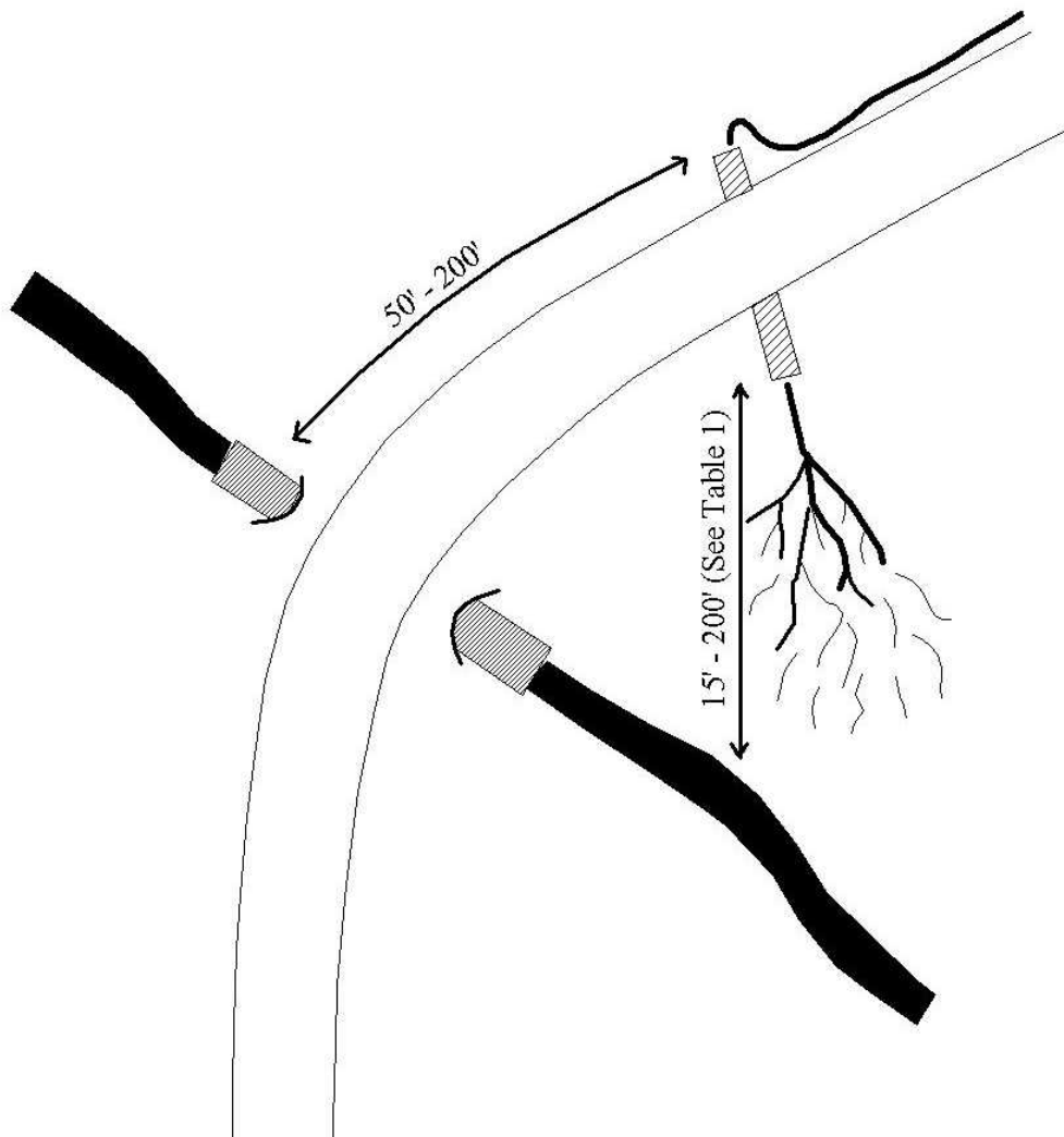
Figure 4. Installation of cross-drains above stream crossings to effectively filter muddy runoff.
