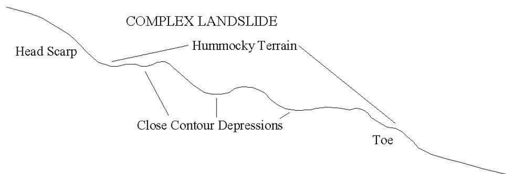
Figure 2. Common ground features of complex landslides; scale on order of thousands of feet.
