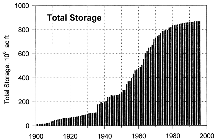
Figure 3. Graph showing the increasing cumulative storage capacity behind dams in the United States, 1900–1996. The most rapid increase was between about 1950 and 1970, with the end of the dam building era by about 1980. Data from U.S. Army Corps of Engineers (1996); figure design from Graf (1999).
