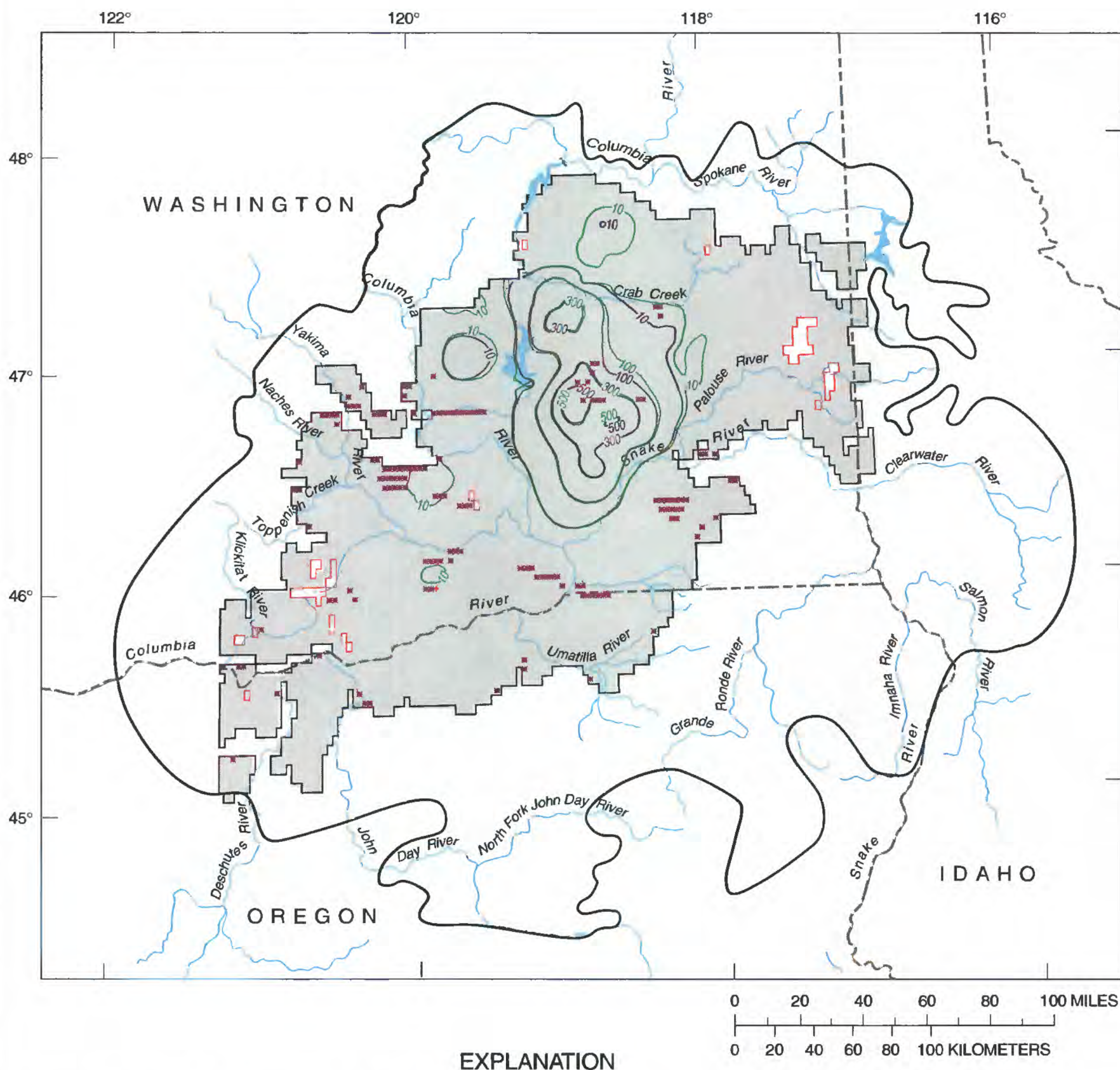
Figure 20. Simulated water-level rises in the Wanapum unit under future equilibrium conditions resulting from the proposed expansion of the Columbia Basin Irrigation Project, Phases 1 and 2.
