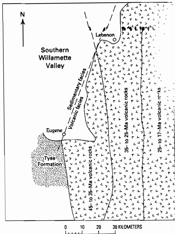
Figure 96. Map showing outcrop belts of western Cascade Range volcanic rocks (modified from Sherrod and Pickthorn, 1989) and the north-northeast-trending boundary between volcanic and sedimentary rocks (dashed line). The facies boundary controls the position of the eastern edge of the Willamette Valley; erosionally resistant volcanic rocks are to the east-southeast and weak sedimentary rocks, principally the Eugene Formation, are to the west-northwest beneath the valley.
