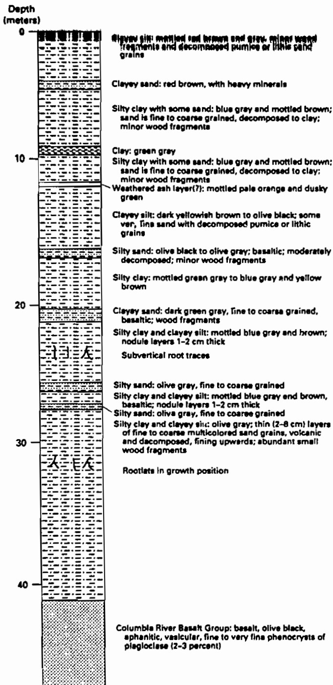
Figure 80. Graphic log of corehole DH 14-90, drilled 1.4 km west of Sublimity at State Highway 22 north of Mill Creek on the south edge of the Waldo Hills, Oregon, showing unnamed nonmarine sedimentary deposits overlying the Columbia River Basalt Group.
