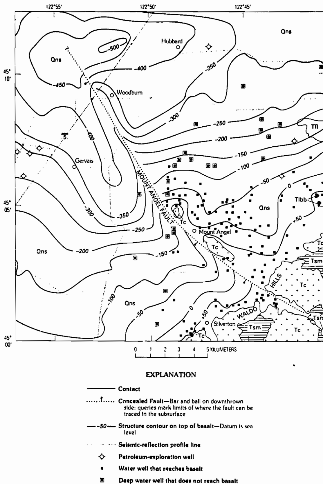
Figure 89. Structure contour map of the top of basalt units near Mount Angel, Oreg. The basalt is primarily the top of the Columbia River Basalt Group except near exposures of the Miocene basalt and basaltic andesite around the Mount Angel fault. Qns, Holocene and Pleistocene nonmarine sedimentary deposits; Tn, Pliocene and Miocene fluvial and lacustrine(?) sedimentary deposits; Tc, Columbia River Basalt Group (Miocene); Tsm, Miocene and Oligocene Scotts Mills Formation of Miller and Orr (1988); Tibb, Miocene basalt and basaltic andesite.
