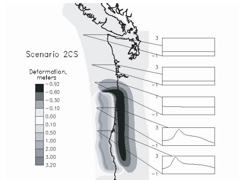
Figure 7: Surface deformation from the least case fault rupture, Scenario 2CS. This rupture is essentially the same as the 2CN case but for a southern segment break on the subduction zone. Figure taken from Myers et al. (1999).
