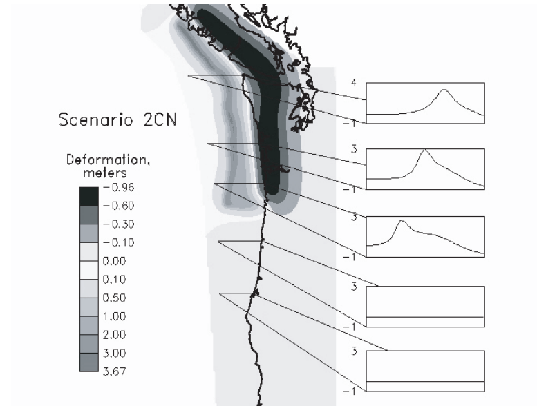
Figure 6: Surface deformation from the least case fault rupture, Scenario 2CN. This rupture is based on half the slip of the Scenario 1A but a maximum rupture width. The wider rupture was chosen because, other things being equal, wider ruptures produce smaller tsunamis than narrow ruptures in this geologic setting; hence, both slip and width favor smaller tsunamis. The maximum width was based on observations of paleo-coseismic subsidence (Priest et al. , 1997).
