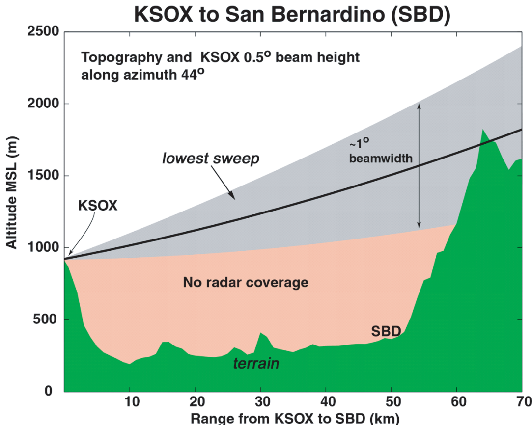
Figure 9. Vertical section of radar coverage across the Los Angeles Basin area.
