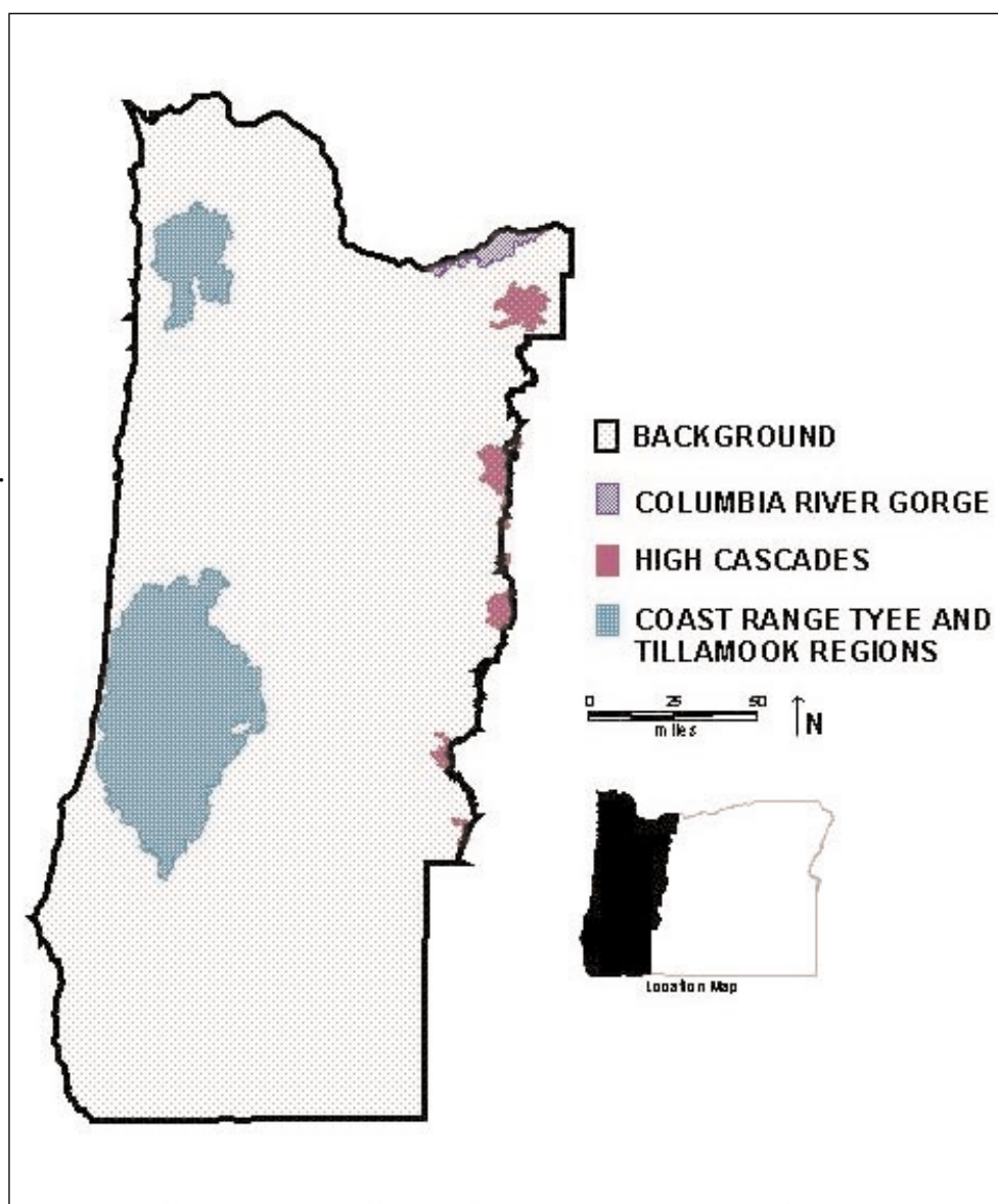
Figure 21. Generalized geographic separation used for selecting deposition hazard cutoff values.
