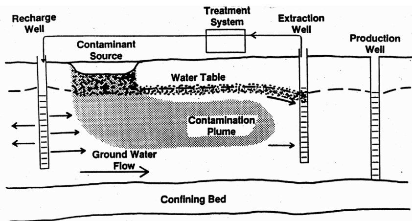
Fig. 12.1 Pump-and-treat system
