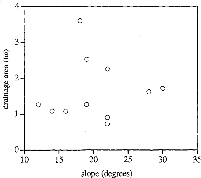
Figure 5. Slope-Drainage Area Relationship for Headwater Streams Mapped in Lookout Creek. No statistically significant relationship is evident for the mapped sites ( Y = 0.009X + 1.5 , p = 0.87 , R^2 = 0.33 ), although there appear to be two marginally significant subgroups of channel heads with drainage areas < 1.1 ha and > 1.6 ha. To delineate the stream network on the digital elevation model, we therefore used a constant source area of slightly less than 2 hectares, roughly approximating the average source area of mapped channels.
