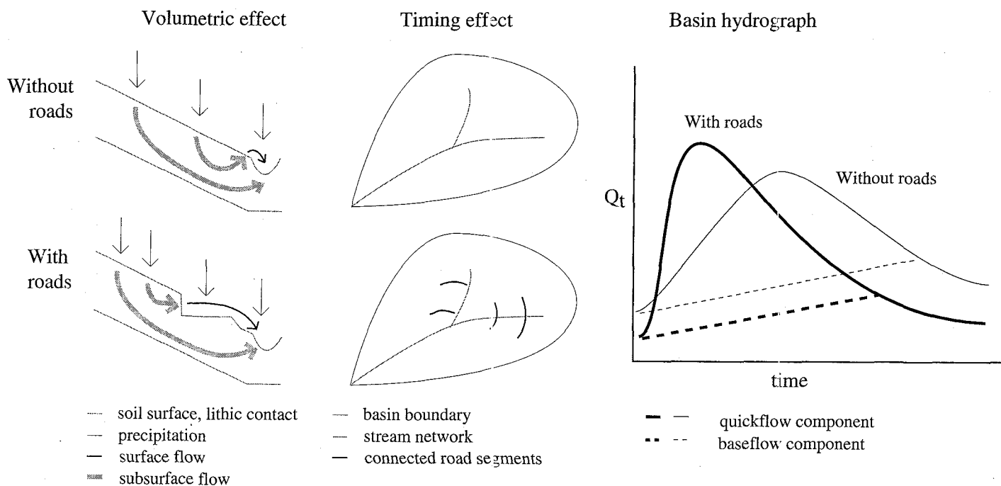
Figure 1. A Conceptual Model of the Hydrologic Function of Roads Based on Two Effects: (1) a volumetric effect, increasing the total volume of water available for quickflow; and (2) a timing effect, altering the flow routing efficiency through extensions to the drainage network (see text).
