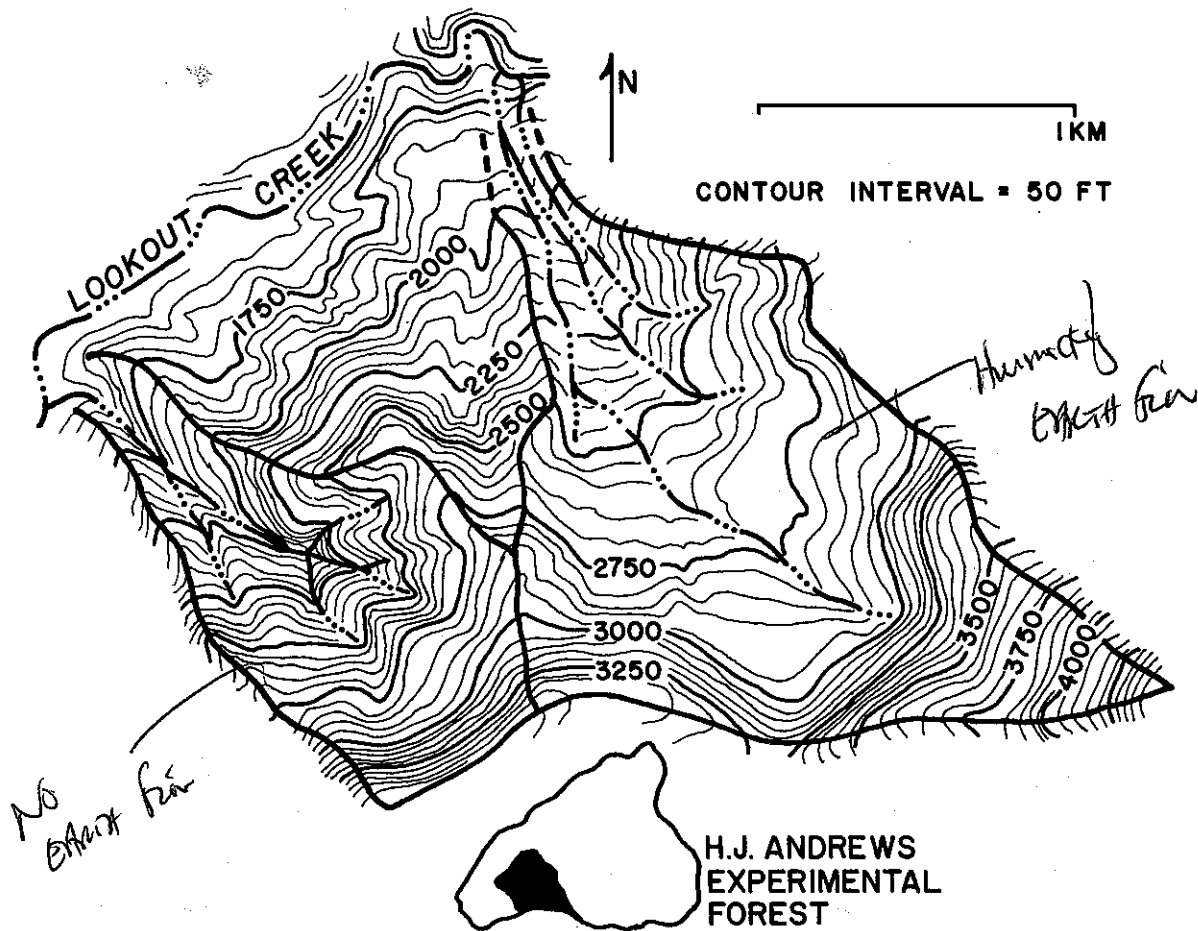
Figure 3.--Topographic map showing contrasting topography between experimental watershed #3 (Fredriksen 1970) on left, which has been deeply dissected by stream erosion and the watershed on right which has undergone deep-seated failure, filling the lower part of the drainage with mass movement material.
