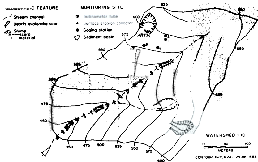
FIGURE 8.3 Geomorphic features and monitoring sites on watershed 10.
