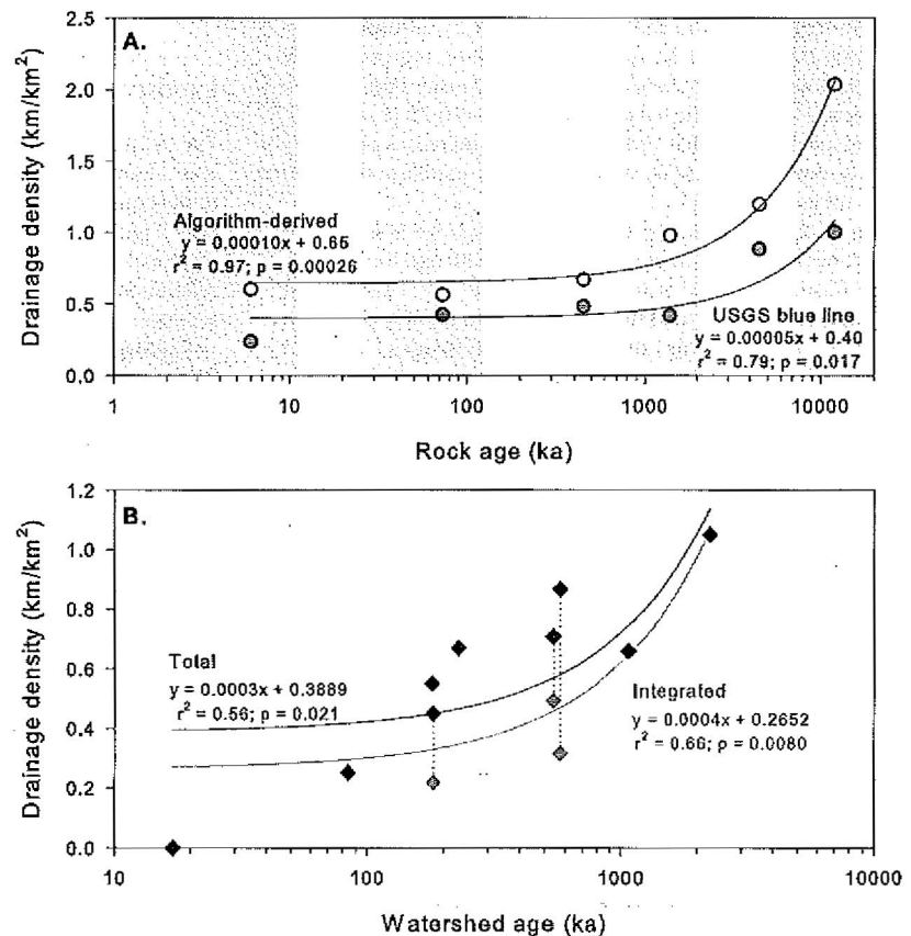
Figure 4. Drainage density versus rock unit and watershed age. (A) Drainage density of basalts and basaltic andesites in the north study area. Stream lengths were measured from digitized 1:24,000 topographic maps (gray circles) and obtained from the valley detection algorithm published by Luo and Stepinski (2008) (white circles). Shaded bars represent the range of ages for map units of Sherrod and Smith (2000), and circles represent the median age of each unit. The regression lines were fitted through the median ages. (B) Black diamonds represent the total drainage density of each study watershed. Gray diamonds represent integrated drainage density of watersheds where integrated drainage density is lower than total drainage density. Integrated drainage density is defined as the length of stream connected to the watershed outlet, divided by watershed area. Lengths of streams that drain to closed basin lakes or wetlands are not counted in the integrated drainage density calculation. Dashed lines show the relationship between total drainage density and integrated drainage density for specific watersheds.
