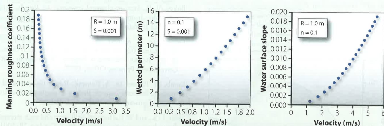
Graphs showing the relationship between velocity and changing values of the Manning roughness coefficient, channel wetted perimeter, and water surface slope.
