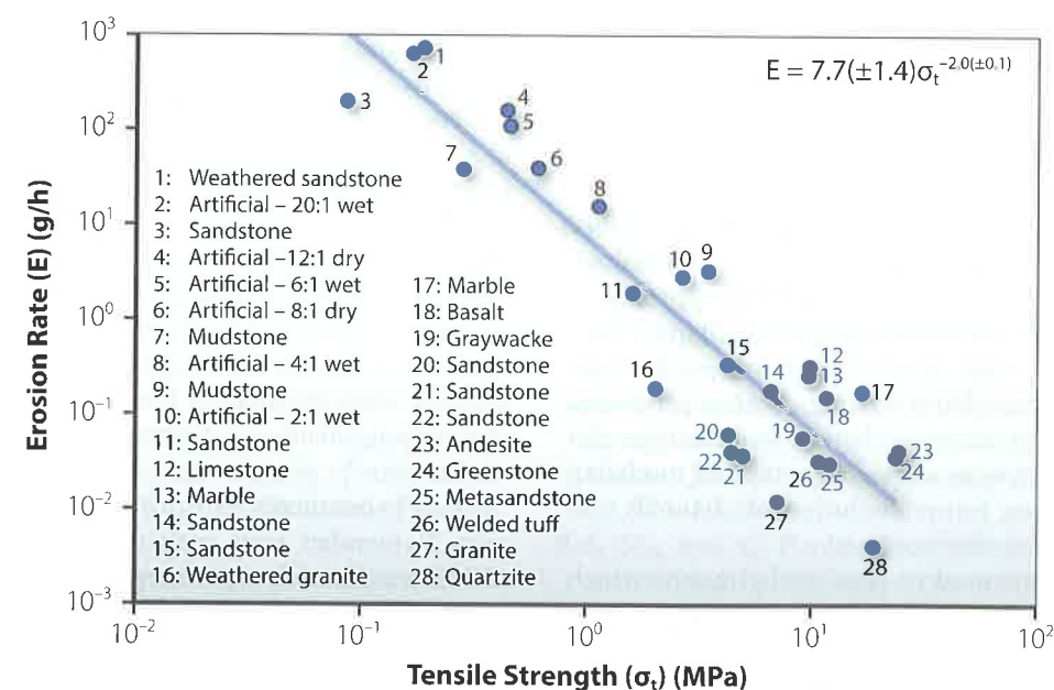
FIGURE DD6.2 Plot of experimental data from the rock-tumbling experiment described in the text. It shows that the variation in measured erosion rate (expressed in grams per hour) decreases with the square of rock tensile strength. Strong rocks (e.g.,
