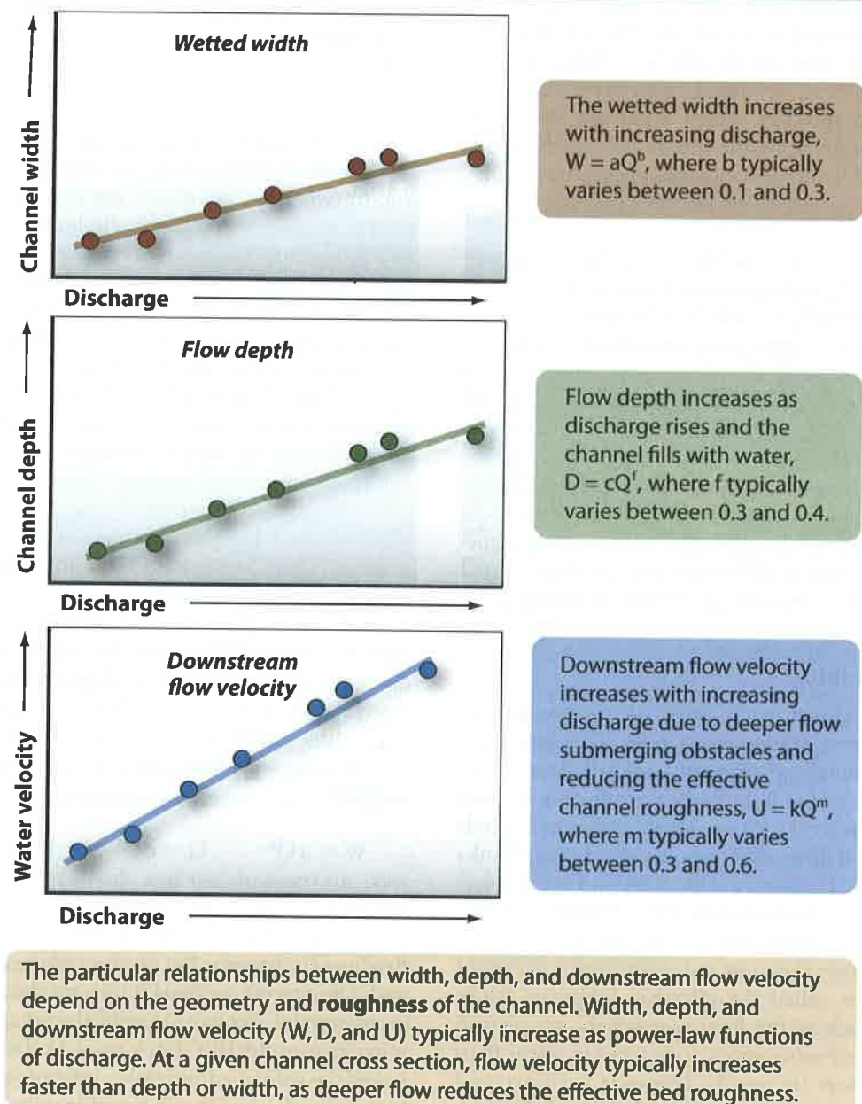
FIGURE 6.2 At-A-Station Hydraulic Geometry. The hydraulic geometry of a channel cross section (at a station) describes the relationships between increasing discharge and the flow width, depth, and velocity.
