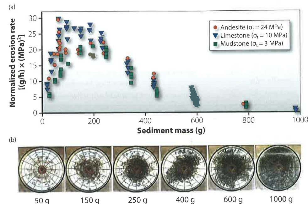
FIGURE DD6.3 (a) The variation in experimental erosion rate (the tumbler, again) with increasing sediment load (mass). Data for three rock types are normalized for rock strength by multiplying erosion rate (expressed in grams per hour) by the square of the rock tensile strength (expressed in megapascals, MPa). (b) A series of photographs taken from below the abrasion mill looking up through the glass bottom. They show how alluvial bed cover increases with increasing sediment loading. [From Sklar and Dietrich (2001).]
