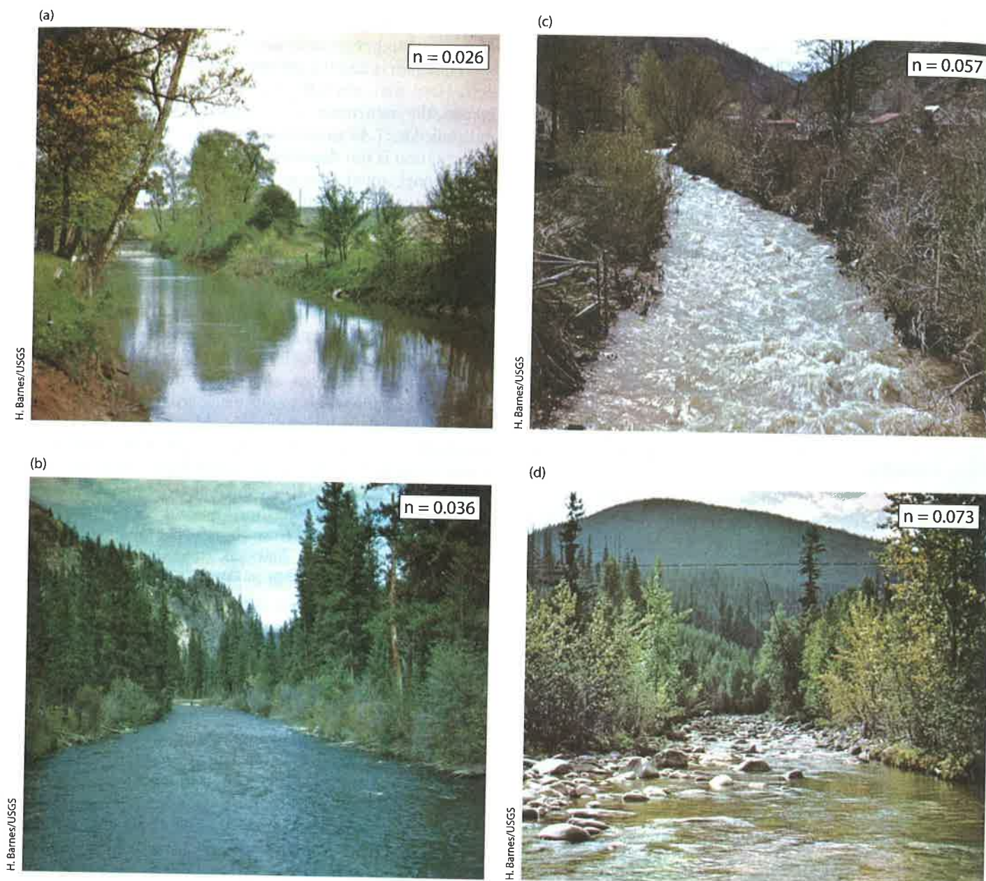
PHOTOGRAPH 6.7 Channel Roughness. Channels have different roughness values, expressed as Manning n values. Images taken from the USGS Water Supply Paper 1849, a compendium of channel roughness values with photographs and cross sections of channels in which the n values were measured. (a) n = 0.026 ,
