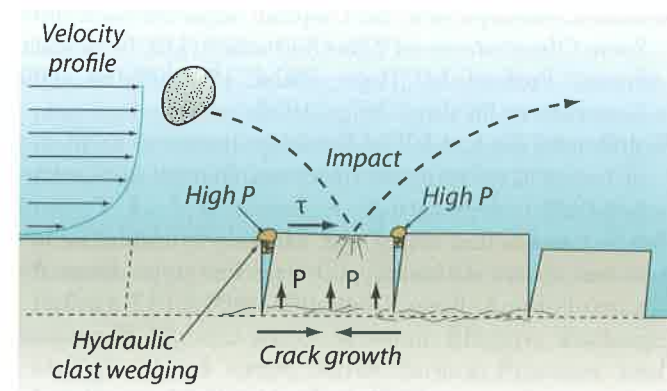
FIGURE DD6.1 Schematic illustration of the processes and forces contributing to bedrock channel erosion by plucking. On the left is the velocity distribution with depth in the channel (arrow length scales relative velocity). Impacts by large saltating grains (shaded) generate stresses that drive the crack propagation necessary to loosen joint blocks. High pressures ( P ) that develop across crack openings in the bed help drive hydraulic wedging of clasts into fractures that work to further open cracks. Surface drag forces due to shear stress ( \tau ) and differential pressures (high P at the surface versus low P at depth) act to lift loosened blocks from the bed. Where the downstream neighbor of a block has been removed, both rotation and sliding become possible, and it is then much easier for rocks to be plucked out of the riverbed. [From Whipple et al. (2000).]
