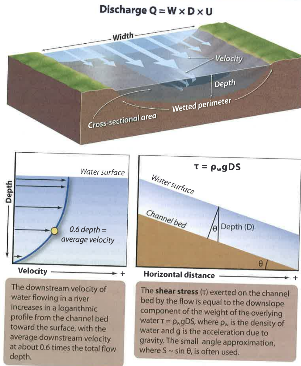
FIGURE 6.1 Channel Cross Section. Channel characteristics, including depth, width, slope, and water velocity, are measured
