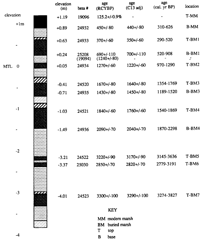
Fig. 12. Core log and radiocarbon ages from core sites 5 and 11. Buried marsh horizons range in radiocarbon age before present (RCYBP) from about 400 to 3300 RCYBP. Radiocarbon dating was performed by Beta Analytic Incorporated (beta #), and standard pretreatment leaches to remove potential contaminants were used. Peat ages were adjusted by 12 C/ 13 C ratios and all ages were calibrated by 14 C reservoir fluctuations. Calibrated ages are based on sample two-sigma deviations about 14 C calibration curves established from tree ring dating [Stuiver and Reimer, 1986].
