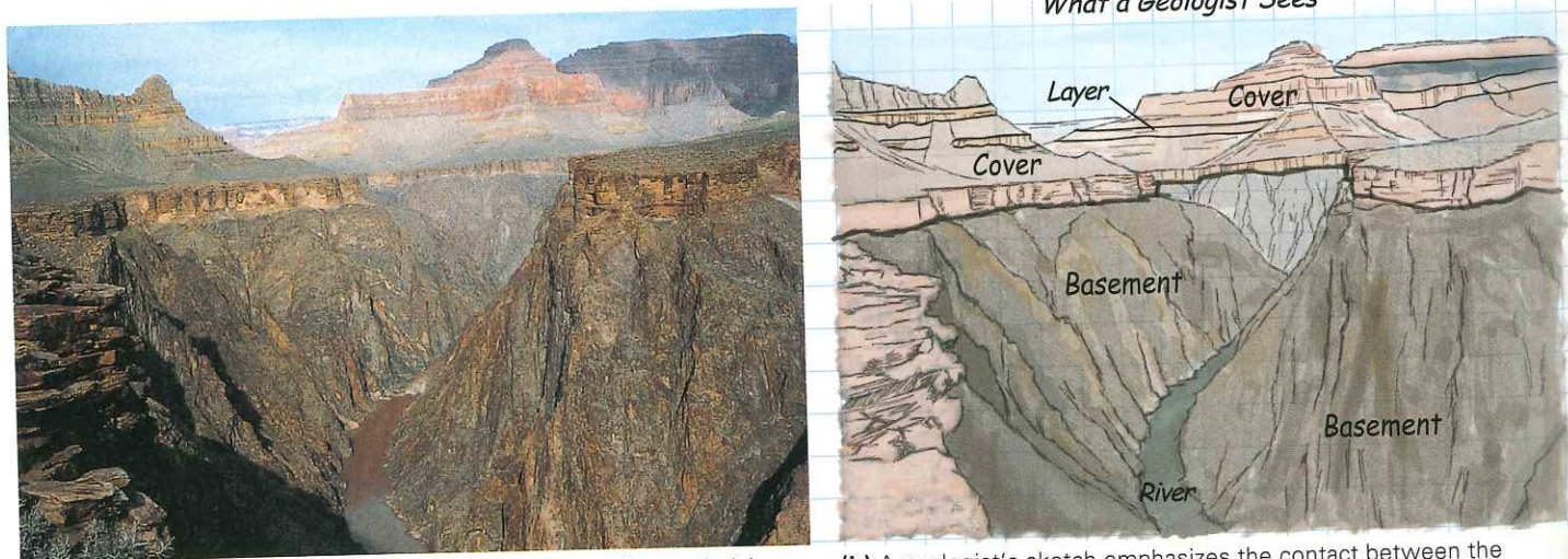
(a) Sedimentary cover here consists of horizontal layers but underlying metamorphic basement does not.
