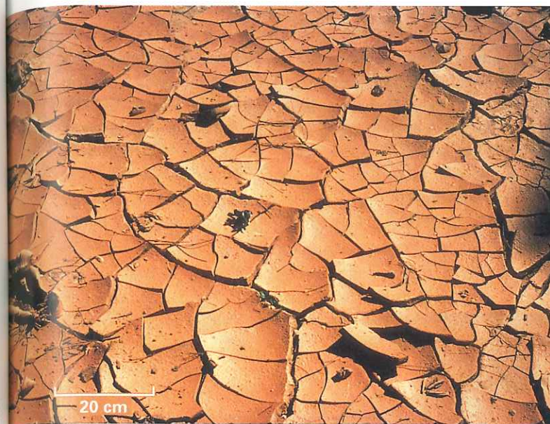
(a) Mud cracks in red mud at Bryce Canyon, Utah. Note how the edges of the mud plates curl up.
