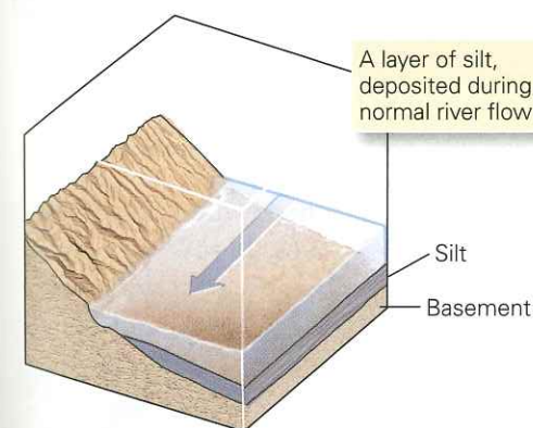
FIGURE 6.10 Bedding in sedimentary rocks.
