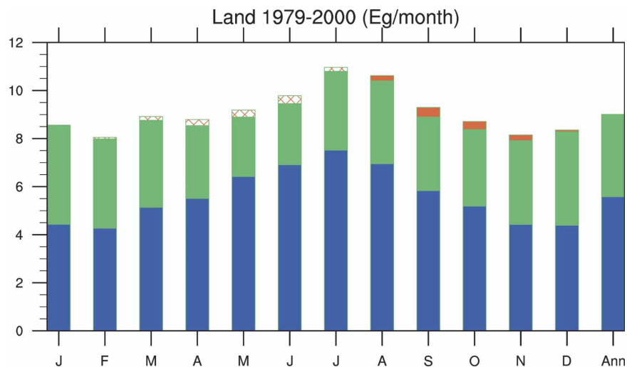
FIG. 4. Annual cycle of moisture budget for global land, ( \text{Eg month}^{-1} ) for 1979–2000. Given are the mean evaporation (blue), inferred column-integrated convergence of atmospheric moisture (green), minus the change in atmospheric storage (red) and total precipitation P as the sum of these P = E - \nabla \cdot \mathbf{Q} - \Delta S at the top of the solid colors. Values that take moisture away from precipitation are cross hatched. The annual mean is given at right (multiply by 12 to get annual value).
