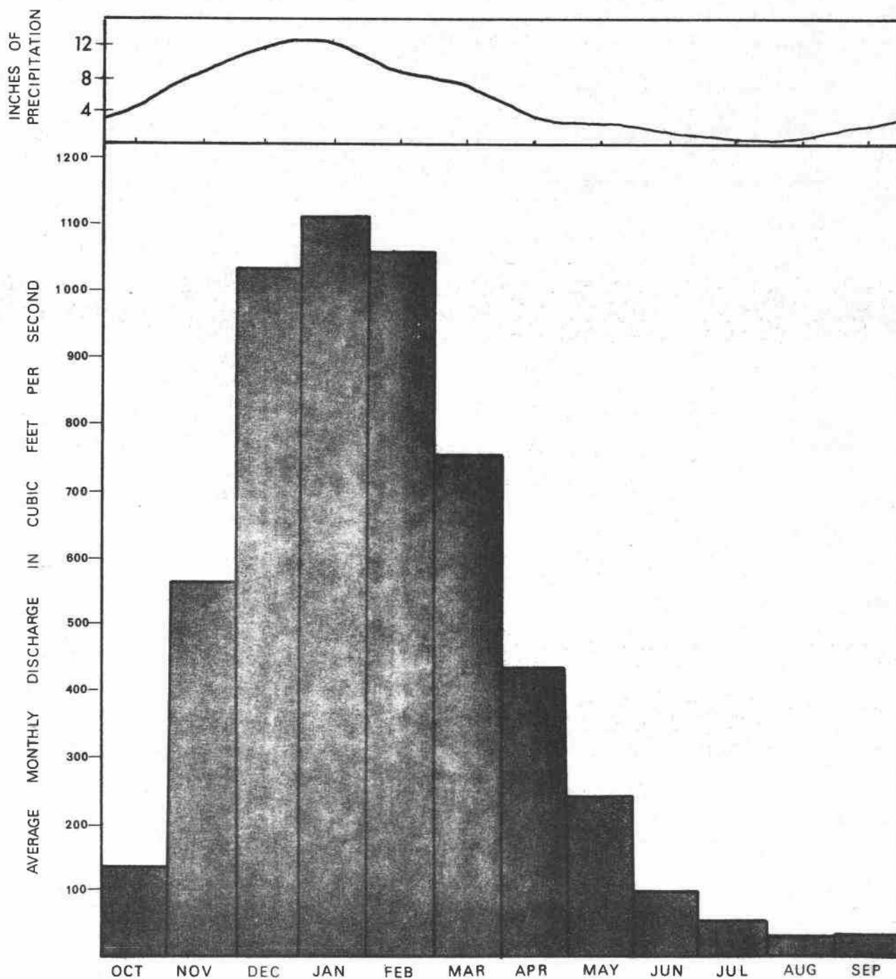
Figure 5. Average monthly precipitation for the years 1857-64 and 1944-54. Average monthly discharge of the Luckiamute River near Pedee, Oregon for the water years 1941-68.
