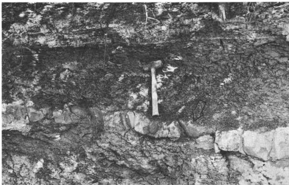
Figure 8. Bedded Kings Valley Siltstone with thin light-colored tuff lamina ( ← ) and thicker resistant basaltic sandstone rib ( → ) (east stream bank of the Luckiamute River near Kings Valley cemetery). One-foot hammer for scale.
