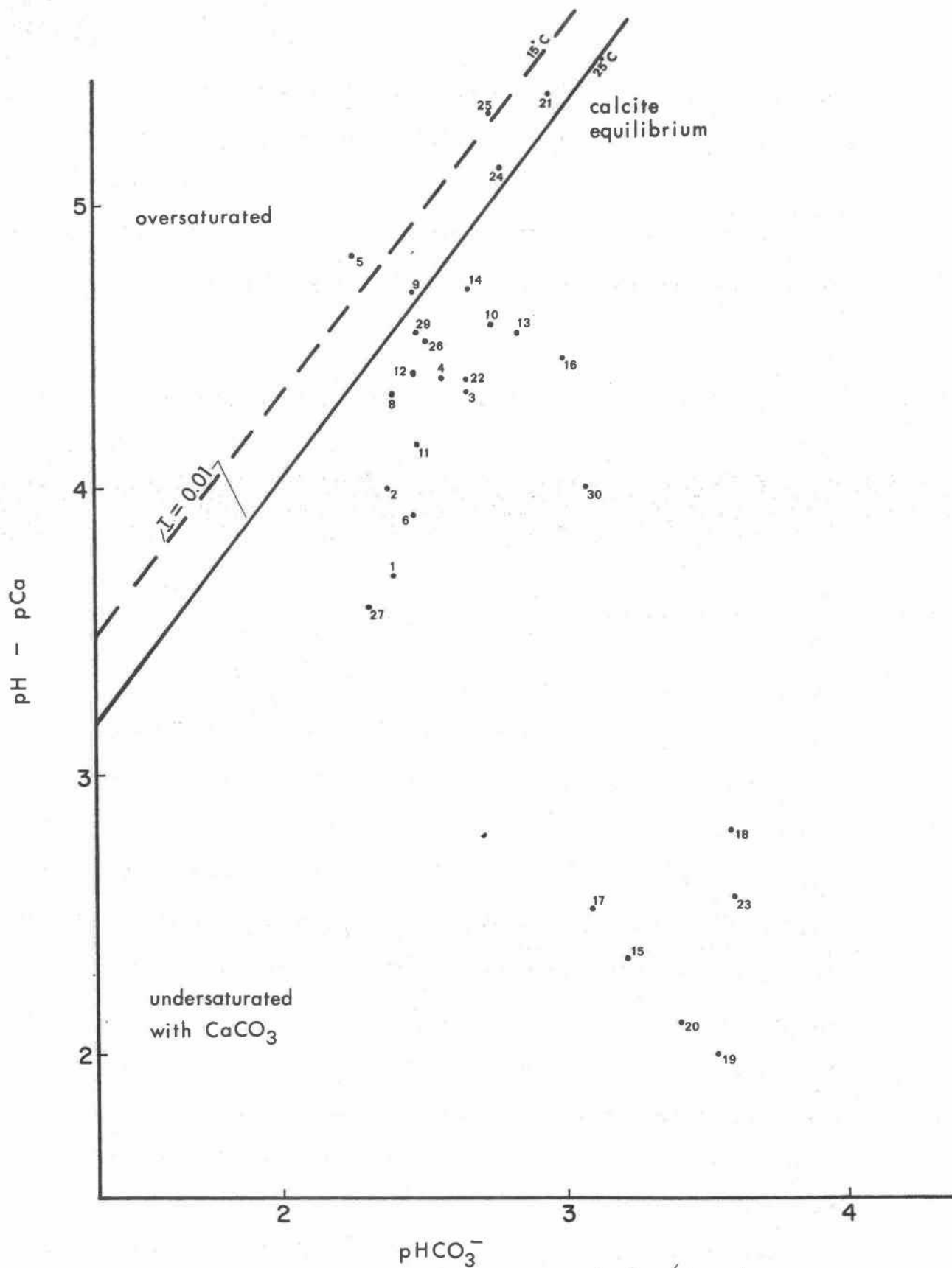
Figure 17. Calcite equilibrium diagram. \frac{[H^+]}{[Ca^{++}]} is plotted as a function of [HCO_3^-] in terms of their negative log concentrations. I=0.01 is the ionic strength and 25^\circ\text{C} is the temperature of the solution for which the calcite equilibrium condition is defined (after Stumm and Morgan, 1970, p. 410).
