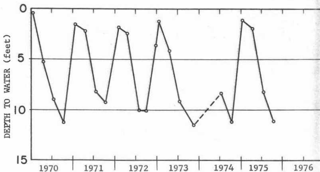
Figure 15. Hydrograph of well 10S/6W-21abb in Kings Valley Siltstone for the period 1970-75.
