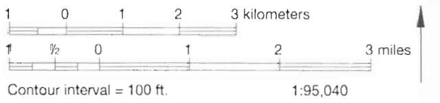
FIGURE 12.14: Mt. Rainier, Washington
