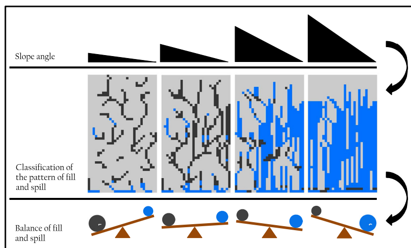
Figure 6. A classification of fill and spill from the surface in Figures 3 and 5. Lateral connectivity can be conceptualized as a balance of upslope accumulated area (black pixels) and downslope drainage efficiency (denoted by blue pixels). Where the slope is low, the accumulated patches of saturation are large but poorly connected as fill (F) dominates spill (S). As the macroscale slope steepens to the right-hand side, spill dominates over fill and water streams down the ‘surface’; micro and mesotopography become less significant. Modified from Hopp and McDonnell (2009)
