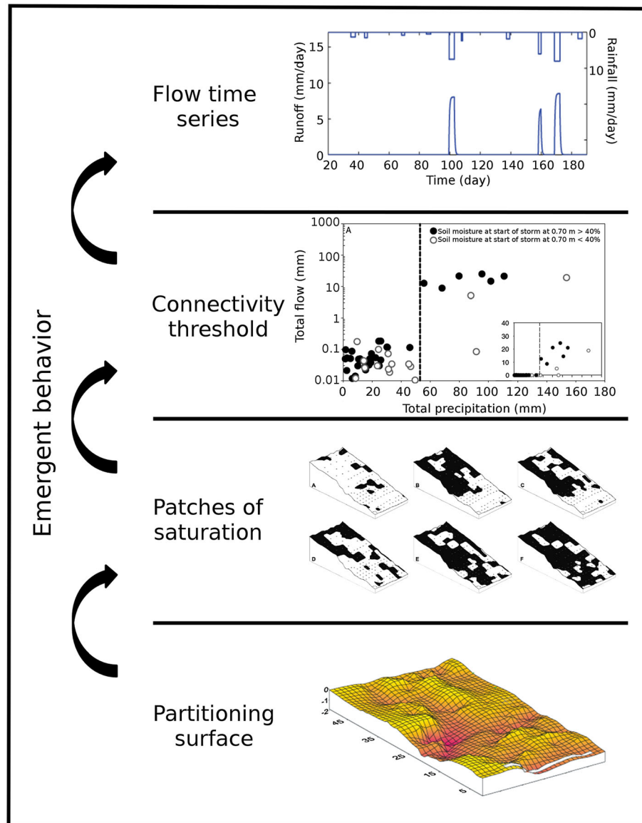
Figure 5. Emergent behaviour from a partitioning surface. The 'surface' may be the soil surface or the soil-bedrock interface or some other subsoil interface. Connectivity may be patches of saturation that are generated at the soil surface or in the subsurface at a subsurface interface by infiltration excess or saturation excess. In addition to all runoff processes being the same, all runoff processes have filling, spilling, transmission losses, connectivity and thresholds at their core. Modified from the original diagram developed by Ciaran Harman, Johns Hopkins University, with his figure based on plots from Freer et al. (2002) and Tromp-van Meerveld and McDonnell (2006a,b) and modified from its use in Troch et al. (2009)
