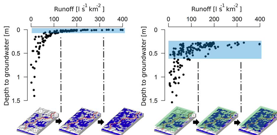
Figure 4. Conceptual rendering of saturation excess overland flow (a) and its subsurface counterpart (b) with data modified from Seibert et al. (2003). The time series of saturated patch connectivity is from the modeling of Frei et al. (2010), who showed striking similar behaviour for saturation excess as seen earlier by Tromp-van Meerveld and McDonnell (2006a) and shown in Figure 3
