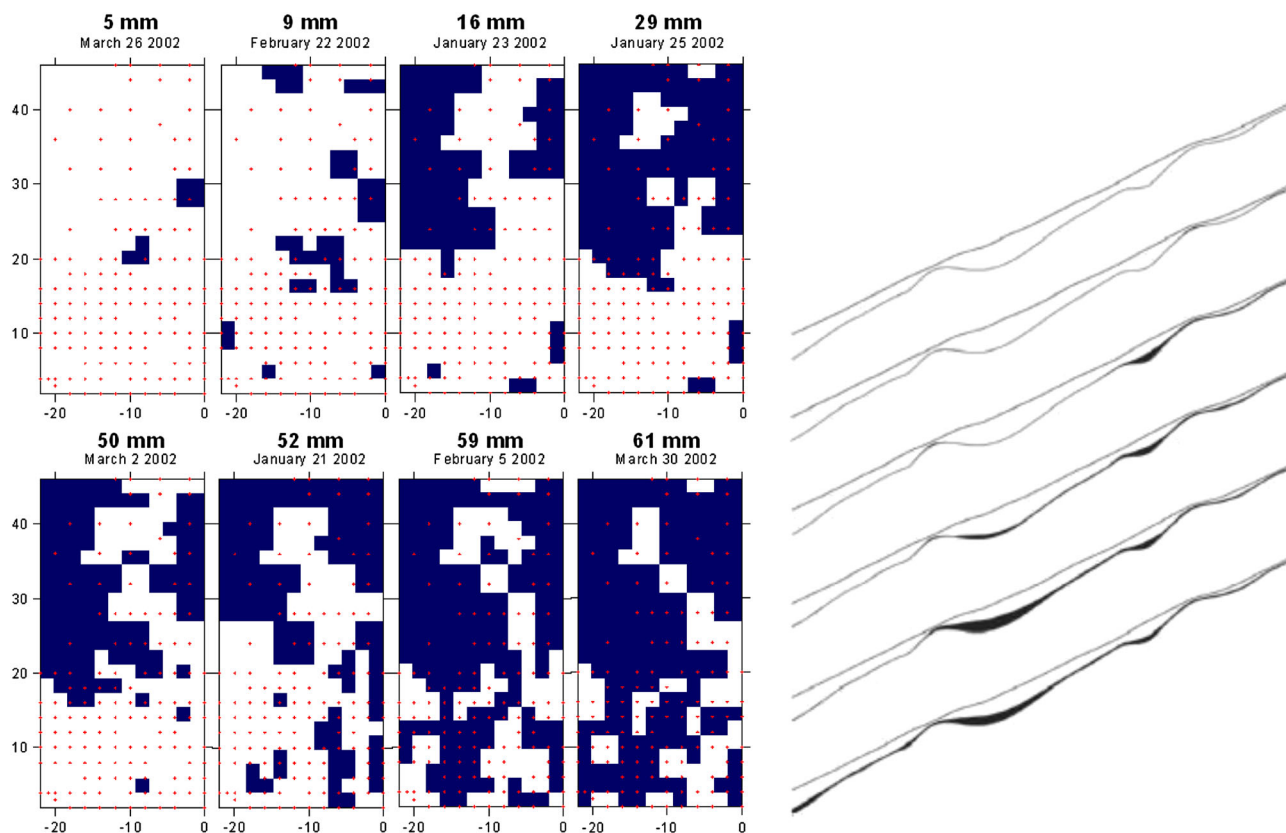
Figure 3. Fill and spill behaviour from a forested hillslope in Georgia, USA. Ponding produced by infiltration excess at the soil-bedrock interface with growth and later connectivity of saturated patches resulting in threshold runoff behaviour at the slope base. The right-hand side illustrates the same behaviour for a 2D cross section of the slope, showing that such runoff may be produced from the top-down; or from upper soil sections to lower slope sections. Modified from Tromp-van Meerveld and McDonnell (2006b)
