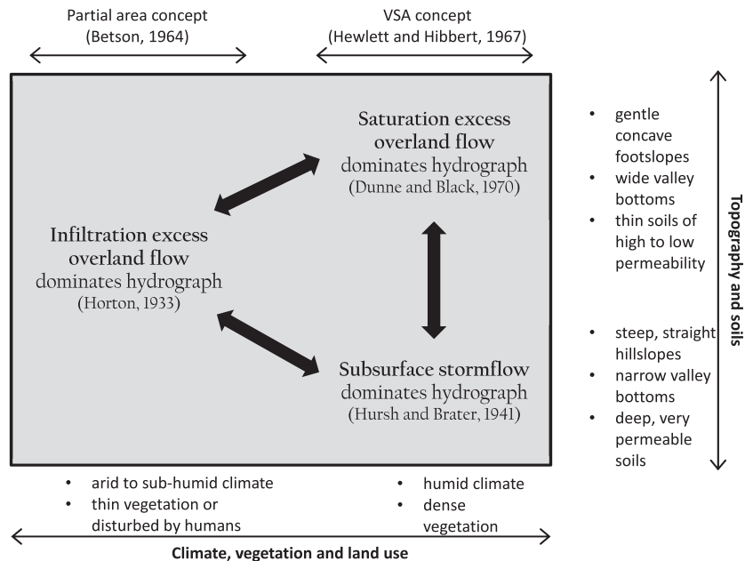
Figure 1. The three runoff classes based on discovery of overland flow from early descriptions of surface runoff due to infiltration excess overland flow (Horton, 1933) to partial area restriction of where infiltration excess can occur (Betson, 1964); to subsurface stormflow controls where all water is assumed to infiltrate to then form lateral flow contribution to channel stormflow (Hursh and Brater, 1941) to saturation excess overland flow (Dunne and Black, 1970), the latter two in the context of variable source area theory. Modified from the original diagram by Dunne (1983)
