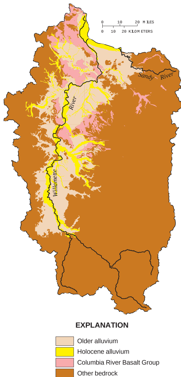
Figure 2. Generalized surficial geology of the Willamette Basin, Oregon. (Modified from Gannett and Caldwell [in press] and Walker and MacLeod [1991].)
