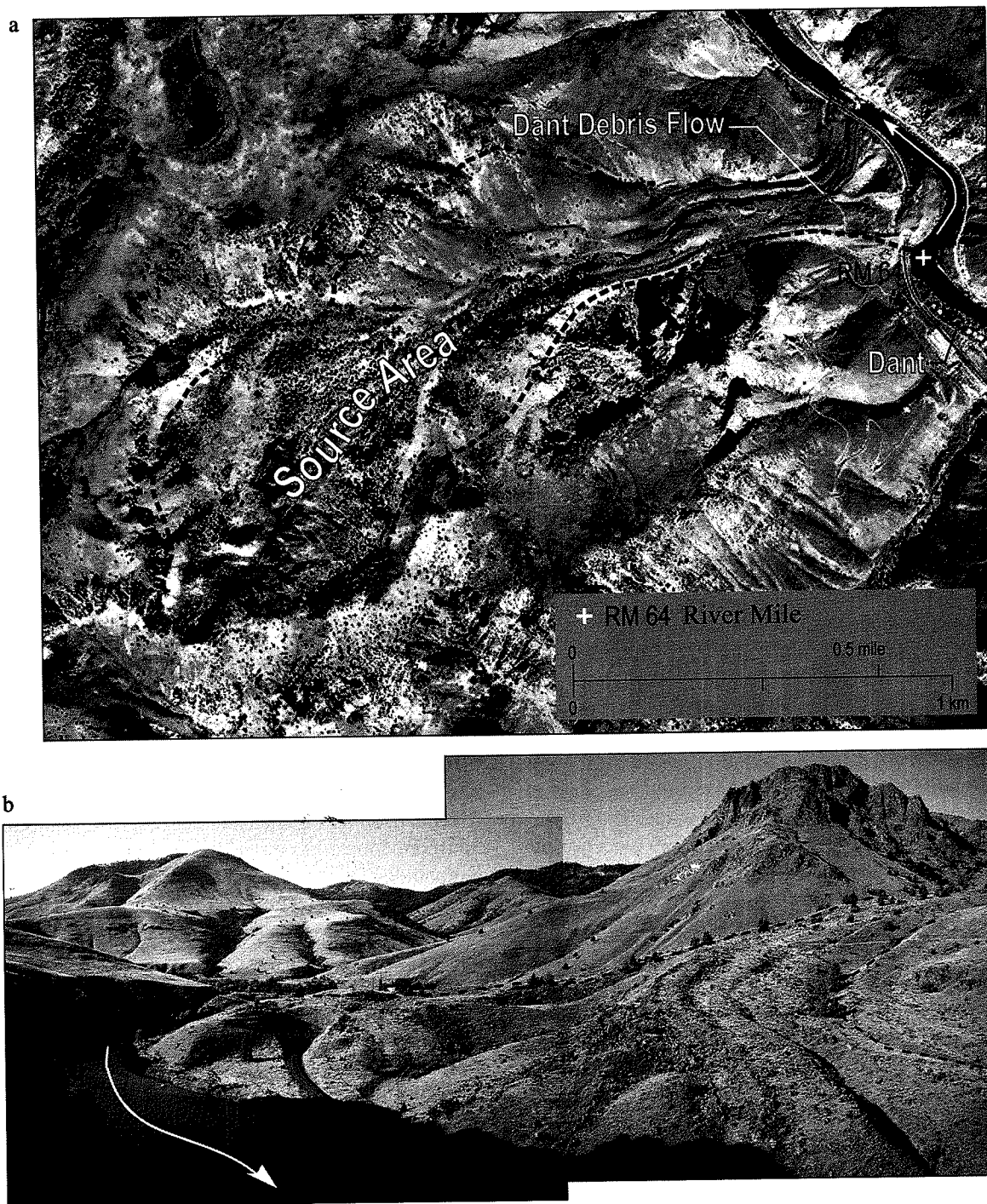
Figure 8. Dant debris flow. (a) Vertical aerial photograph (1995, Portland General Electric) showing flow deposit and inferred source area. (b) Two-photograph panorama directed upstream (south) showing terminus of flow deposit. Railroad and tunnel indicate scale. July 17, 1998, photographs by J. H. Curran.
