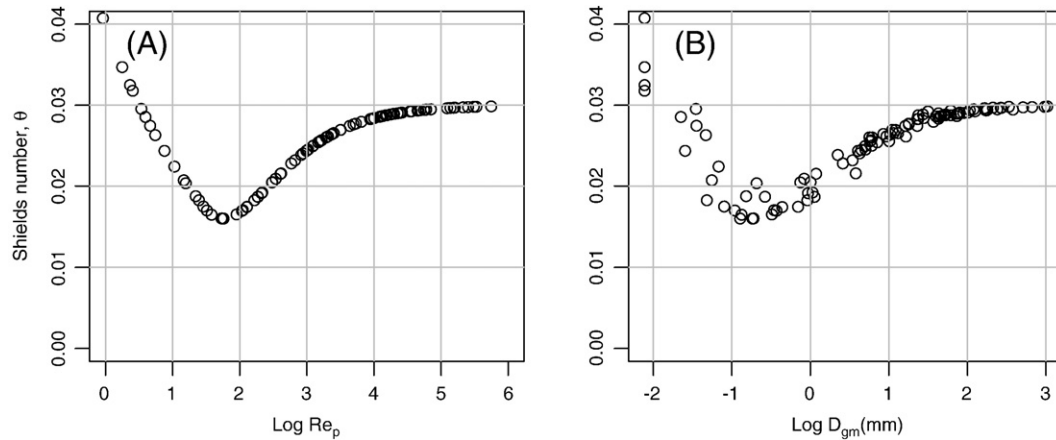
Fig. 3. Shields ratio at incipient motion, \theta , applied in estimating D_{cbf}^* for 104 Oregon and Washington coastal streams sampled in 1994 and 1995, versus (A) Particle Reynolds Number, \text{Log}(\text{Re}_p) , and (B) geometric mean bed surface particle diameter, \text{Log } D_{gm} in mm. Shields ratio was calculated as a function of particle \text{Re}_p at estimated bankfull flow conditions, based on the Equation of Parker et al. (2003) for \text{Re}_p > 26 , and according to our fit to Buffington and Montgomery (1997, plate 1) for \text{Re}_p \leq 26 .
