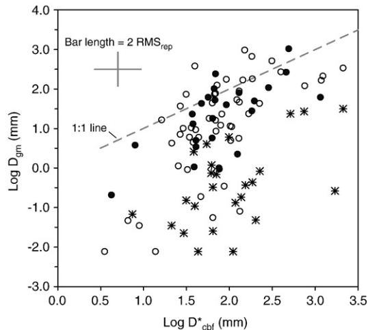
Fig. 7. \text{Log } D_{\text{gm}} vs \text{Log } D^*_{\text{cbf}} in 104 Oregon and Washington coastal streams sampled in 1994 and 1995, showing three levels of basin-riparian disturbance (data from first visit only). Solid circles are sites with the least amount of streamside human land disturbances, the most dense and multi layered corridor of woody riparian vegetation, and the lowest basin road densities ( \text{RCOND} > 0.6 , \text{WRCOND} > 0.6 , and \text{Rd\_Denkm} < 2.0 \text{ km/km}^2 ). Stars are sites with high amounts of human riparian and basin disturbance (i.e., \text{RCOND} < 0.4 , \text{WRCOND} < 0.5 and \text{Rd\_Denkm} > 2.8 \text{ km/km}^2 ). Remaining (medium disturbance) sites are shown as open circles. Length of error bars = 2(\text{RMS}_{\text{rep}}) , where \text{RMS}_{\text{rep}} for \text{Log } D_{\text{gm}} and \text{Log } D^*_{\text{cbf}} are, respectively, 0.43 and 0.27. Dashed line represents D_{\text{gm}} = D^*_{\text{cbf}} (and consequently \text{LRBS}^* = 0 ).
