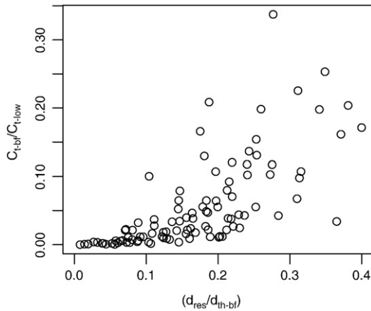
Fig. 4. Ratio of calculated total hydraulic resistance at bankfull flow to that at summer low flow ( C_{t-bf}/C_{t-low} ) versus relative residual depth at bankfull flow ( d_{res}/d_{th-bf} ), a measure of channel form roughness. Data are for 104 Oregon and Washington coastal streams sampled in 1994 and 1995.
