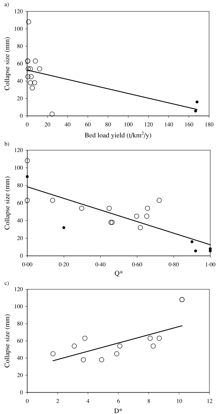
Figure 4. The collapse size decreases with the bed load yield (a) and with Q^* , the degree of supply limitation (b). The collapse size increases with D^* , the degree of selective transport (c). Open circles represent the data from Idaho and the smaller filled circles represent data from elsewhere as described in the text
