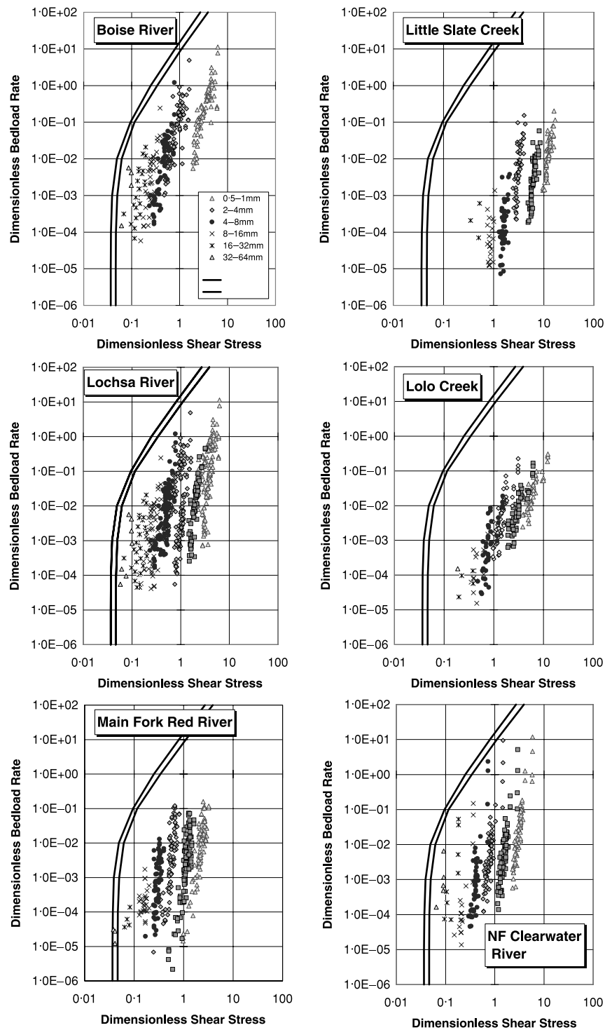
Figure 1. Dimensionless bed load rating curves by particle size class (one-phi interval) for the 12 sites. The two envelope curves encompass the theoretical transport for many bed load equations. The bed load transport rate is weighted by the fraction of the particle size class on the channel bed
