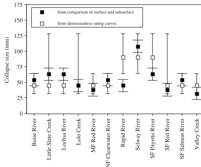
Figure 3. A comparison of the estimates of the upper limit of the supply-limited grain sizes from analysis of the dimensionless bed load rating curves and the comparison of the surface and subsurface size distributions. The geometric mean of the size class approaching the envelope curves is shown by the open square with the error bars at the sieve intervals. For those sites where the value is greater than a particular size, the midpoint of the next size interval is plotted and the upper bound is set at 150 mm. The solid square is the collapse size identified by comparing the surface and subsurface size distributions. The error bars (wide) for the collapse size are arbitrarily set at \pm 10 mm
