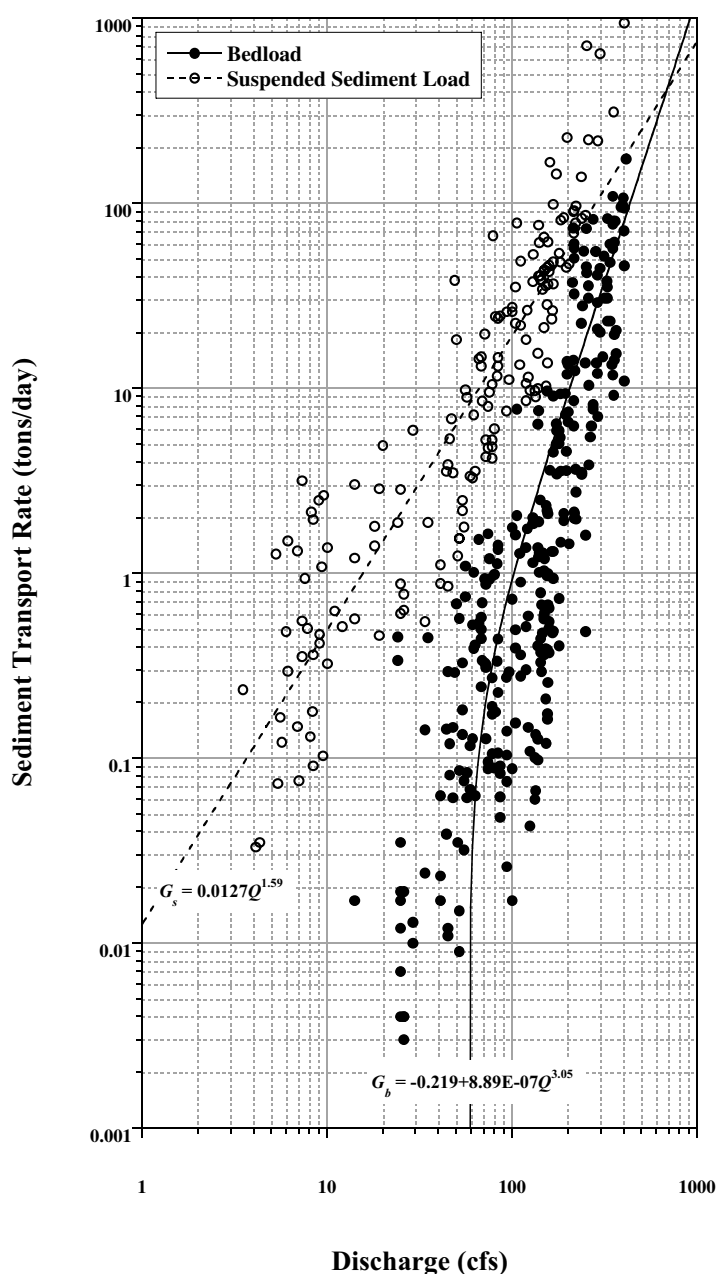
Figure 13 —Comparison between suspended load and bedload measured at Little Granite Creek over the period 1982 through 1997.
