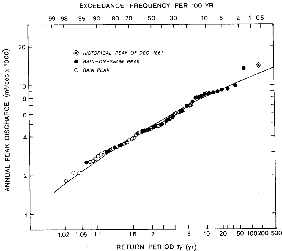
Fig. 5. Historically-weighted, log-Pearson Type-III frequency curve for instantaneous peak flows of the Willamette River at Salem, Oregon, 1814–1977. The historical peak of December 1861 is plotted as the largest in the 164-yr. period. Recorded peaks of 1893–1977 are plotted such that each year represents 1.94 yr. in the 164-yr. period.
