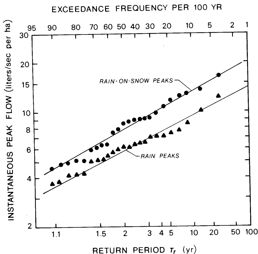
Fig. 7. Frequency curves for peak flows resulting from rain-on-snow and from rainfall at watershed 2, H.J. Andrews Experimental Forest, 1953-1977.
