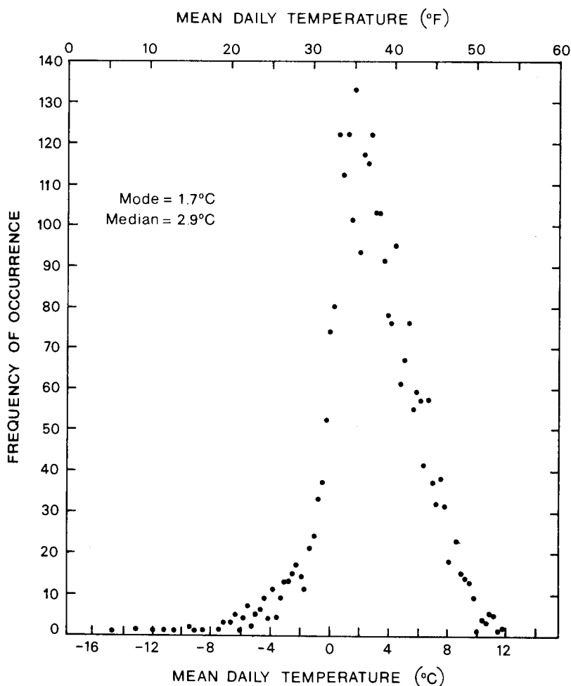
Fig. 12. Frequency distribution of mean daily air temperature T_a at watershed 2 climatic station, H.J. Andrews Experimental Forest, 1958-1977.
