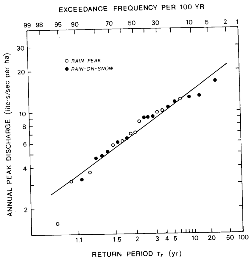
Fig. 6. log-Pearson Type-III frequency curve for peak flows at watershed 2, H.J. Andrews Experimental Forest, 1953-1977.
