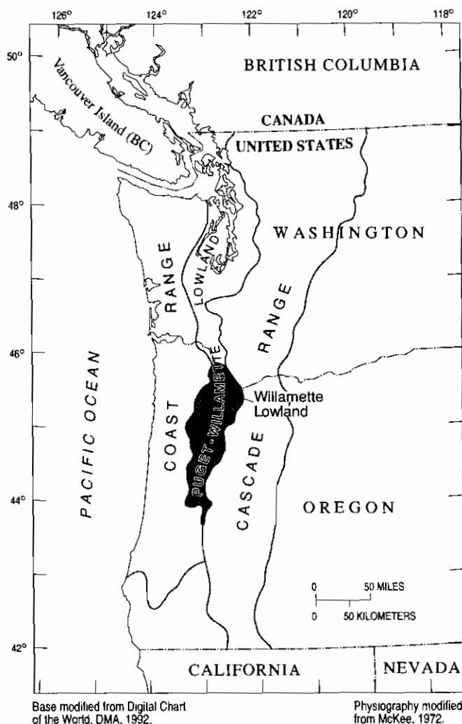
FIGURE 1.—Physiographic setting of the Willamette Lowland.
