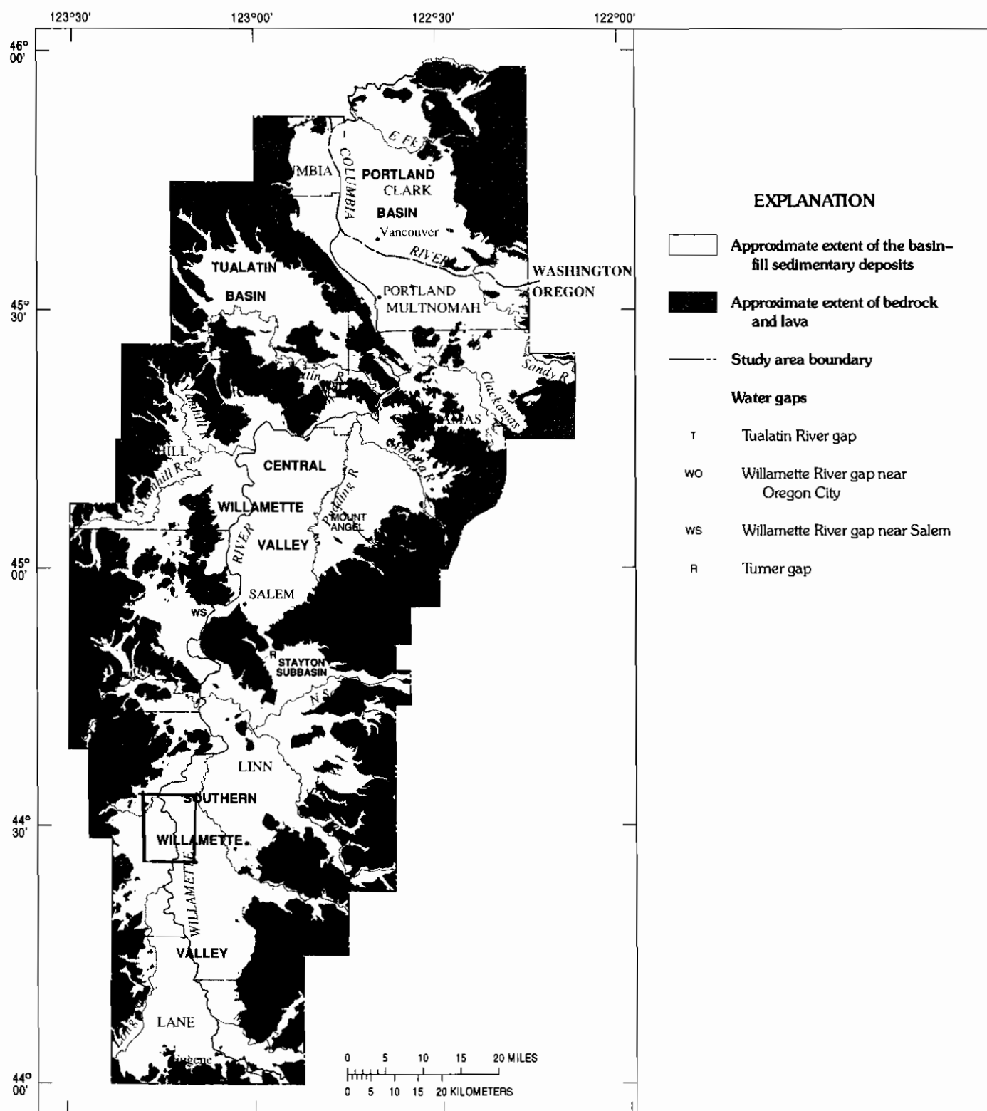
FIGURE 3.—Subbasins and major water gaps within the Willamette Lowland.
