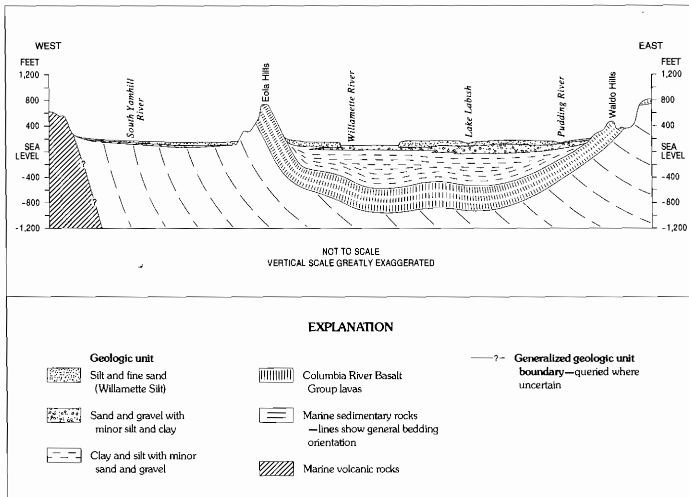
FIGURE 7.—A generalized geologic section west-east through the central Willamette Lowland.
