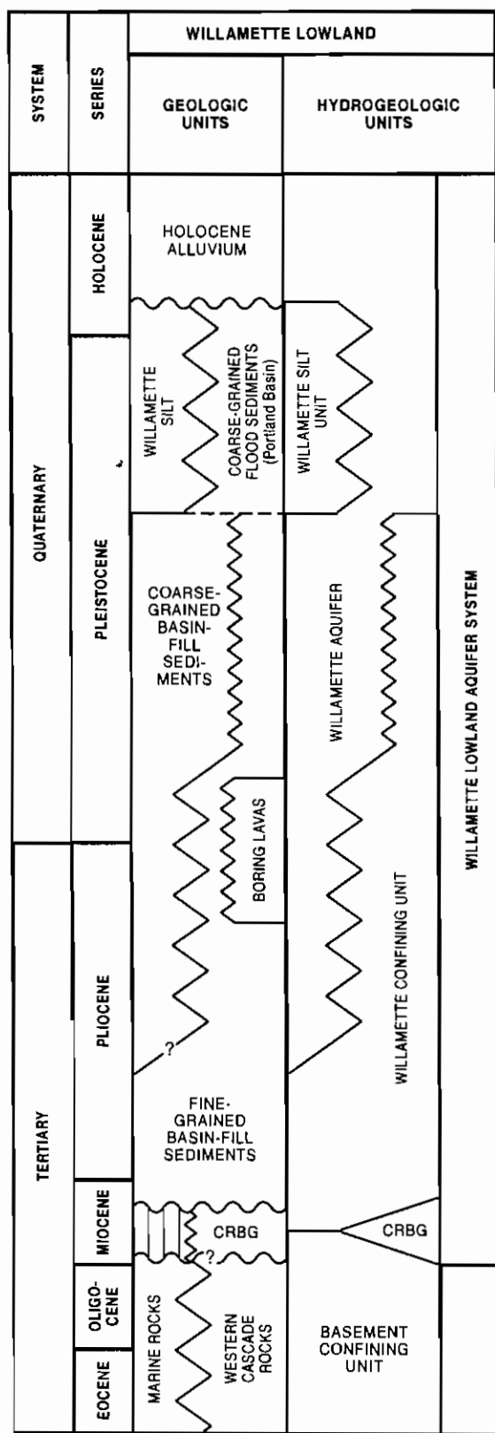
FIGURE 11.—Relation between generalized geologic units and hydrogeologic units in the Willamette Lowland.
