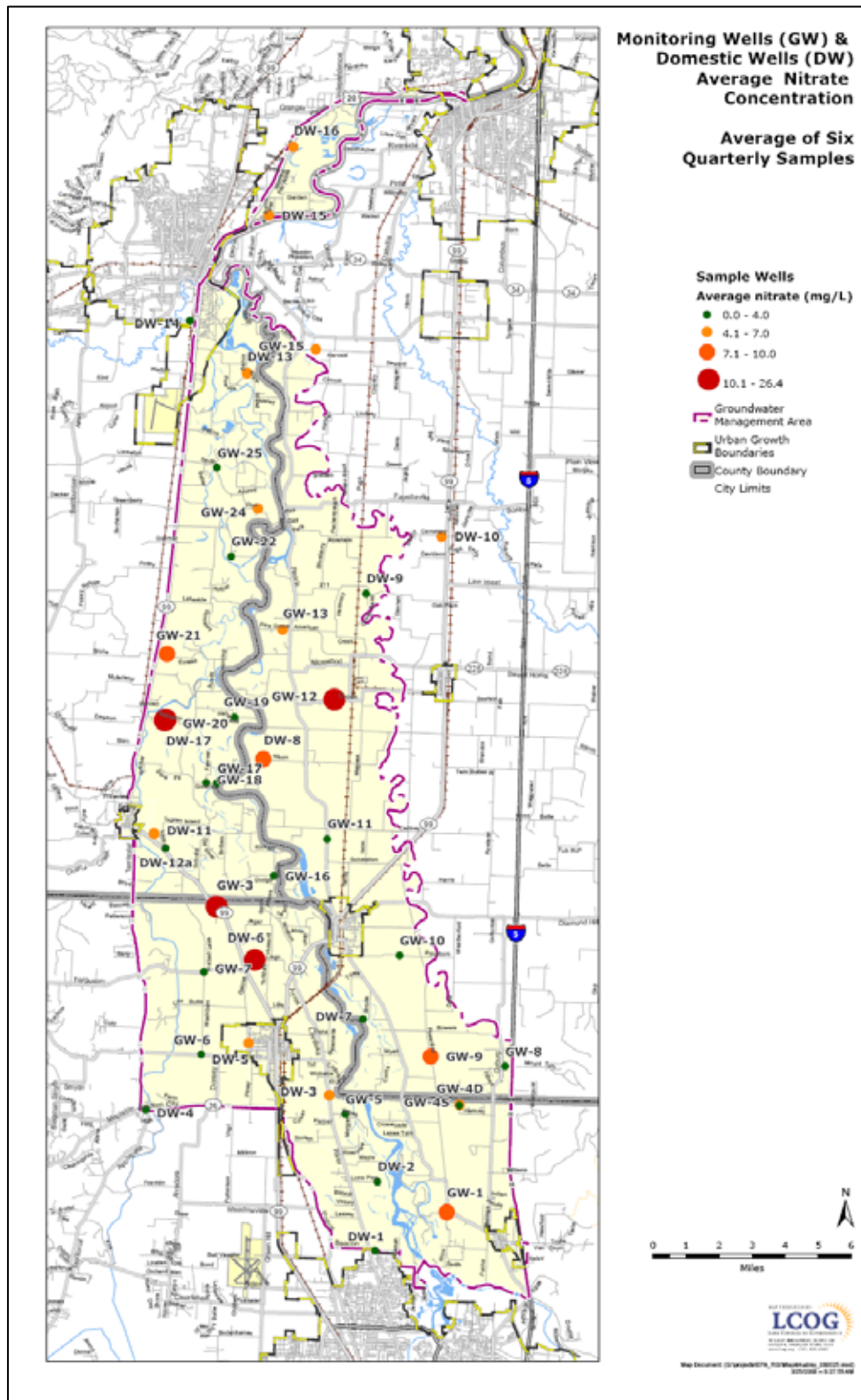
Map 4: Baseline and Long-term Monitoring Sites and Average of First Six Quarters of Nitrate Values In the Groundwater Management Area
