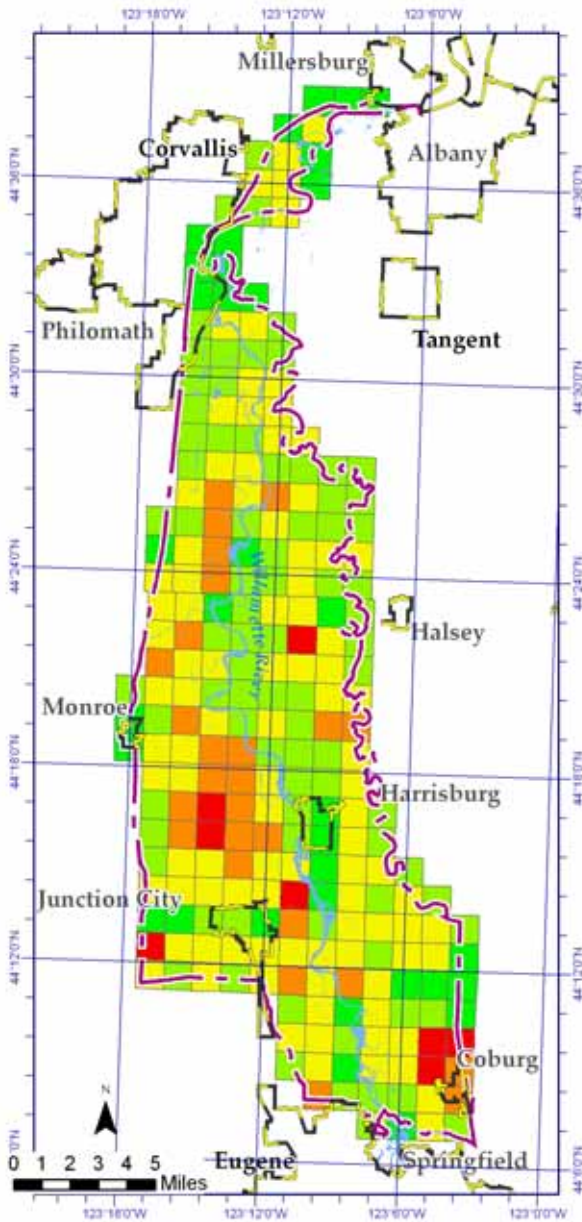
Best Fit Estimated Annual Nitrogen by Section
