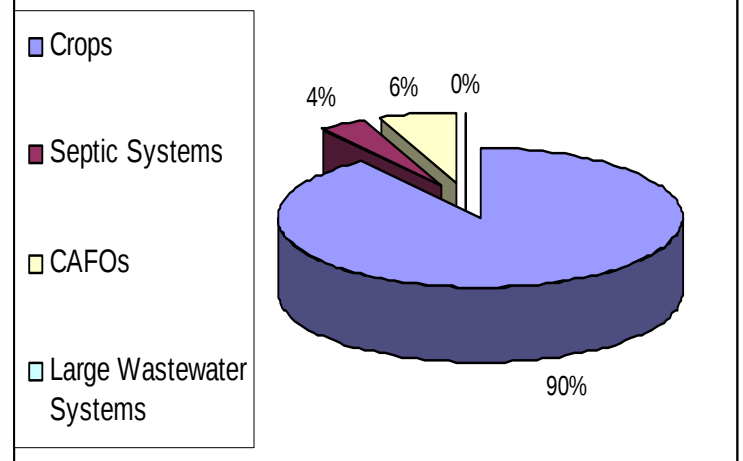
Percentage Nitrogen Contribution by Source
